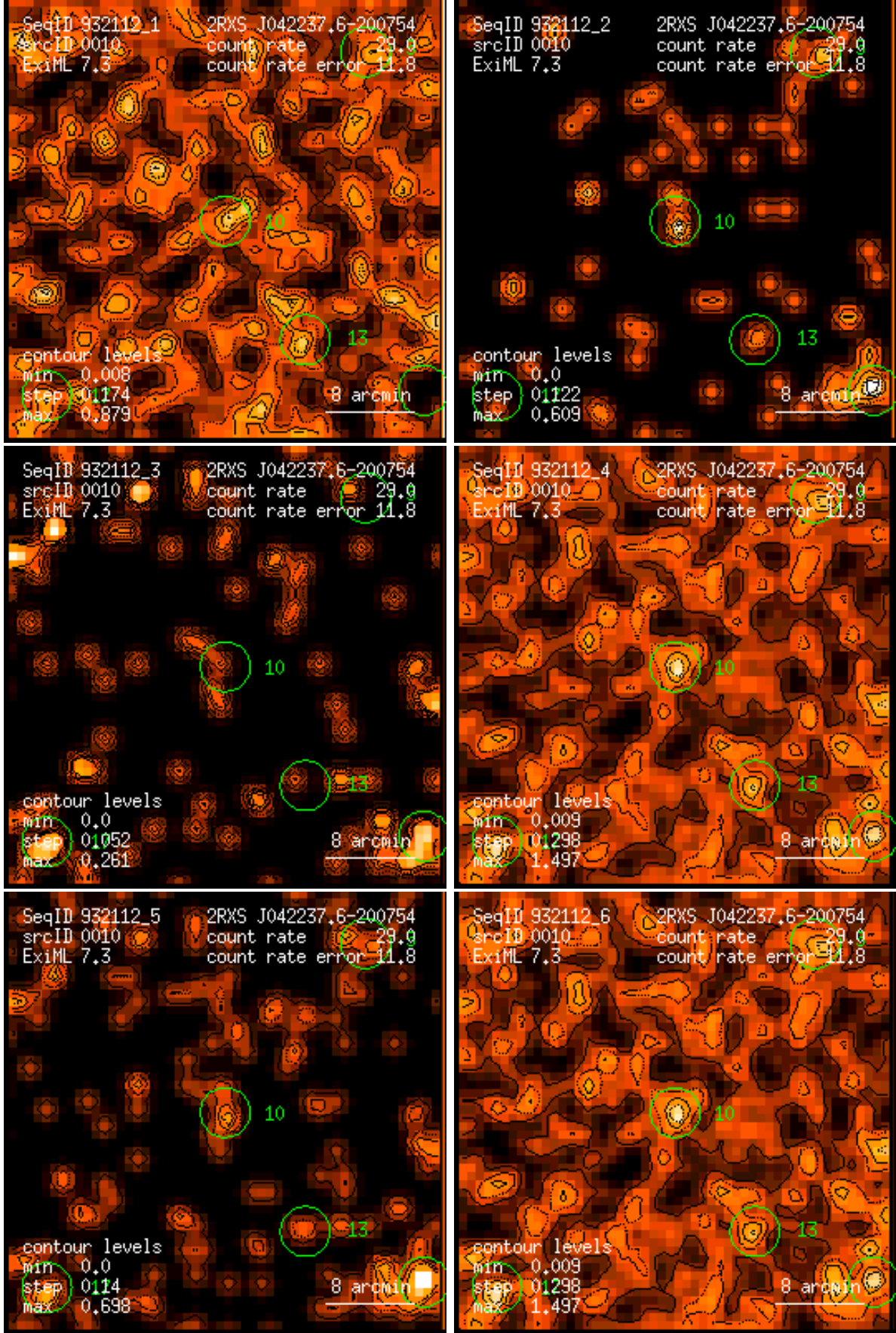
Figure 10: RASS 932112: detection 0010: band rate images, Gaussian filter: (1) PSPC channels 11 – 41, (2) 52 – 90, (3) 91 – 201, (4) 11 – 235, (5) 52 – 201, (6) 11 – 201. Broad band rates in counts/ks. Band rate contour levels in counts/ks/arcmin 2 .
