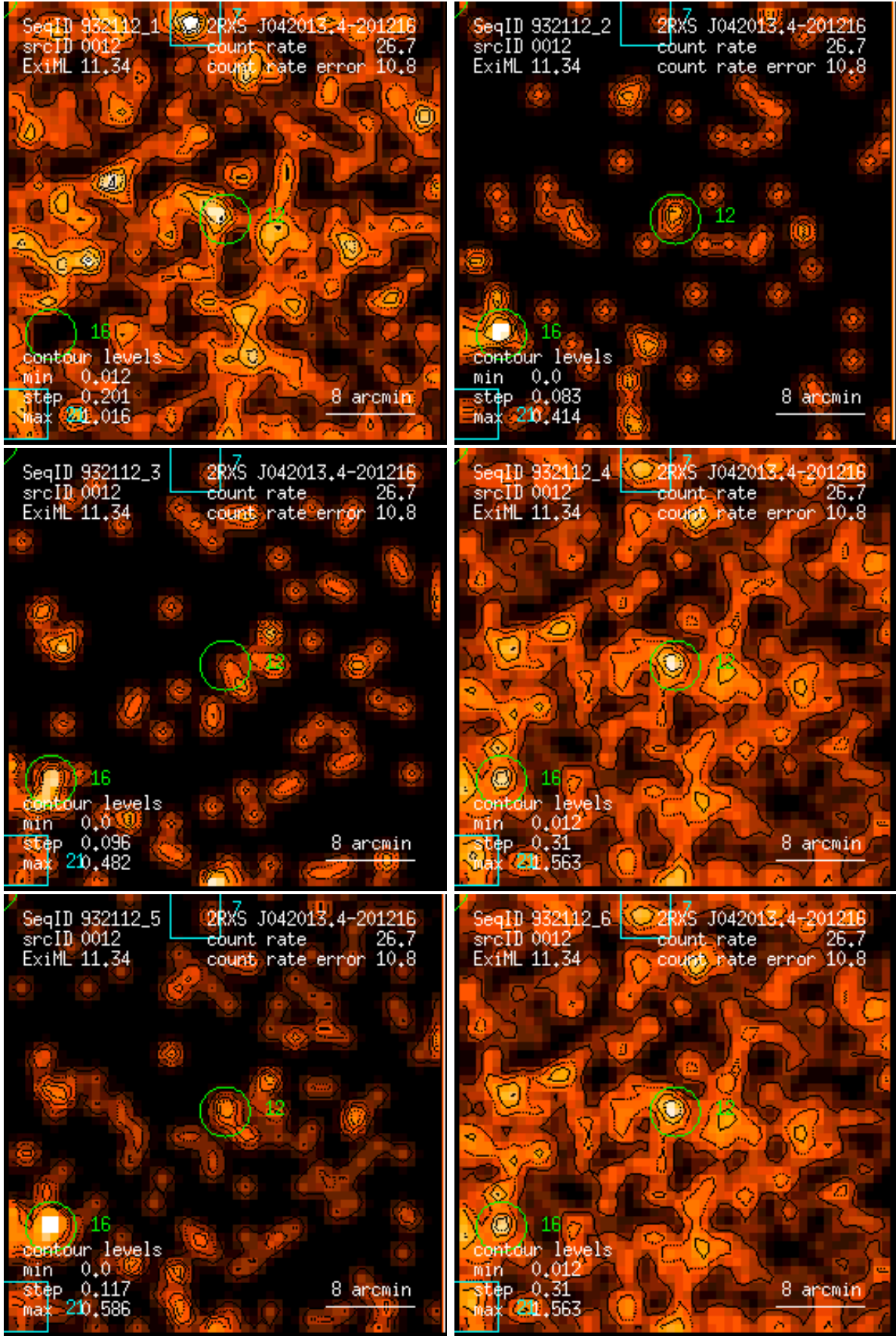
Figure 12: RASS 932112: detection 0012: band rate images, Gaussian filter: (1) PSPC channels 11 – 41, (2) 52 – 90, (3) 91 – 201, (4) 11 – 235, (5) 52 – 201, (6) 11 – 201. Broad band rates in counts/ks. Band rate contour levels in counts/ks/arcmin 2 .
