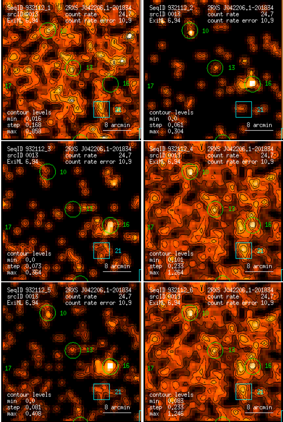
Figure 13: RASS 932112: detection 0013: band rate images, Gaussian filter: (1) PSPC channels 11 – 41, (2) 52 – 90, (3) 91 – 201, (4) 11 – 235, (5) 52 – 201, (6) 11 – 201. Broad band rates in counts/ks. Band rate contour levels in counts/ks/arcmin 2 .
