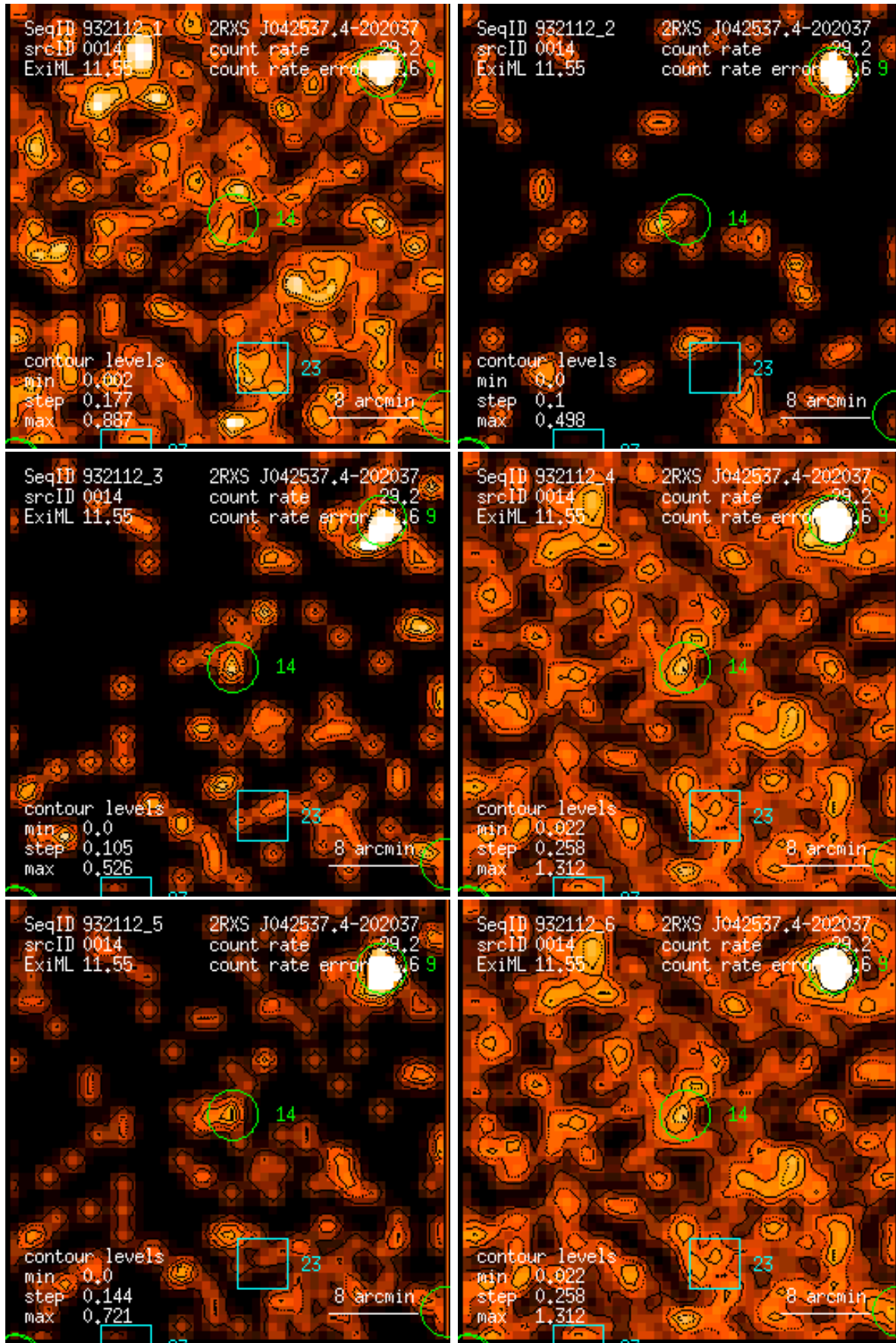
Figure 14: RASS 932112: detection 0014: band rate images, Gaussian filter: (1) PSPC channels 11 – 41, (2) 52 – 90, (3) 91 – 201, (4) 11 – 235, (5) 52 – 201, (6) 11 – 201. Broad band rates in counts/ks. Band rate contour levels in counts/ks/arcmin 2 .
