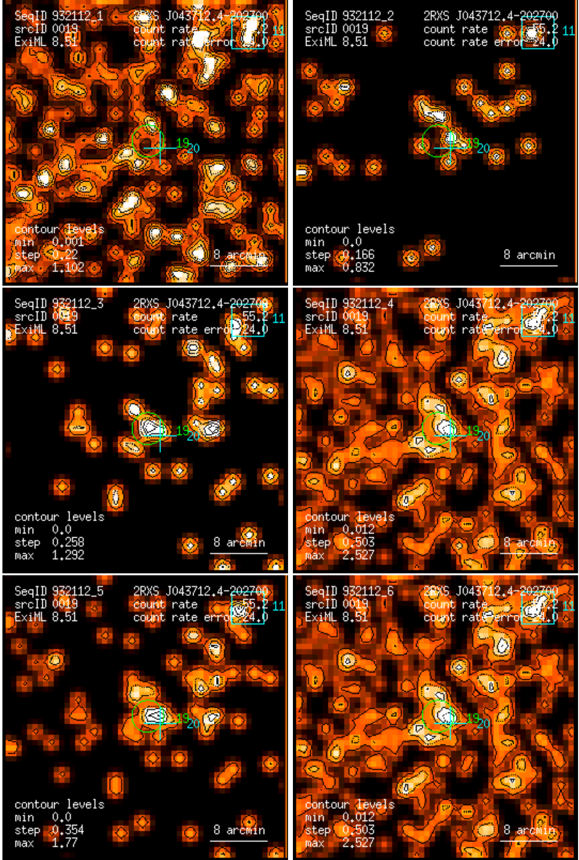
Figure 19: RASS 932112: detection 0019: band rate images, Gaussian filter: (1) PSPC channels 11 – 41, (2) 52 – 90, (3) 91 – 201, (4) 11 – 235, (5) 52 – 201, (6) 11 – 201. Broad band rates in counts/ks. Band rate contour levels in counts/ks/arcmin 2 .
