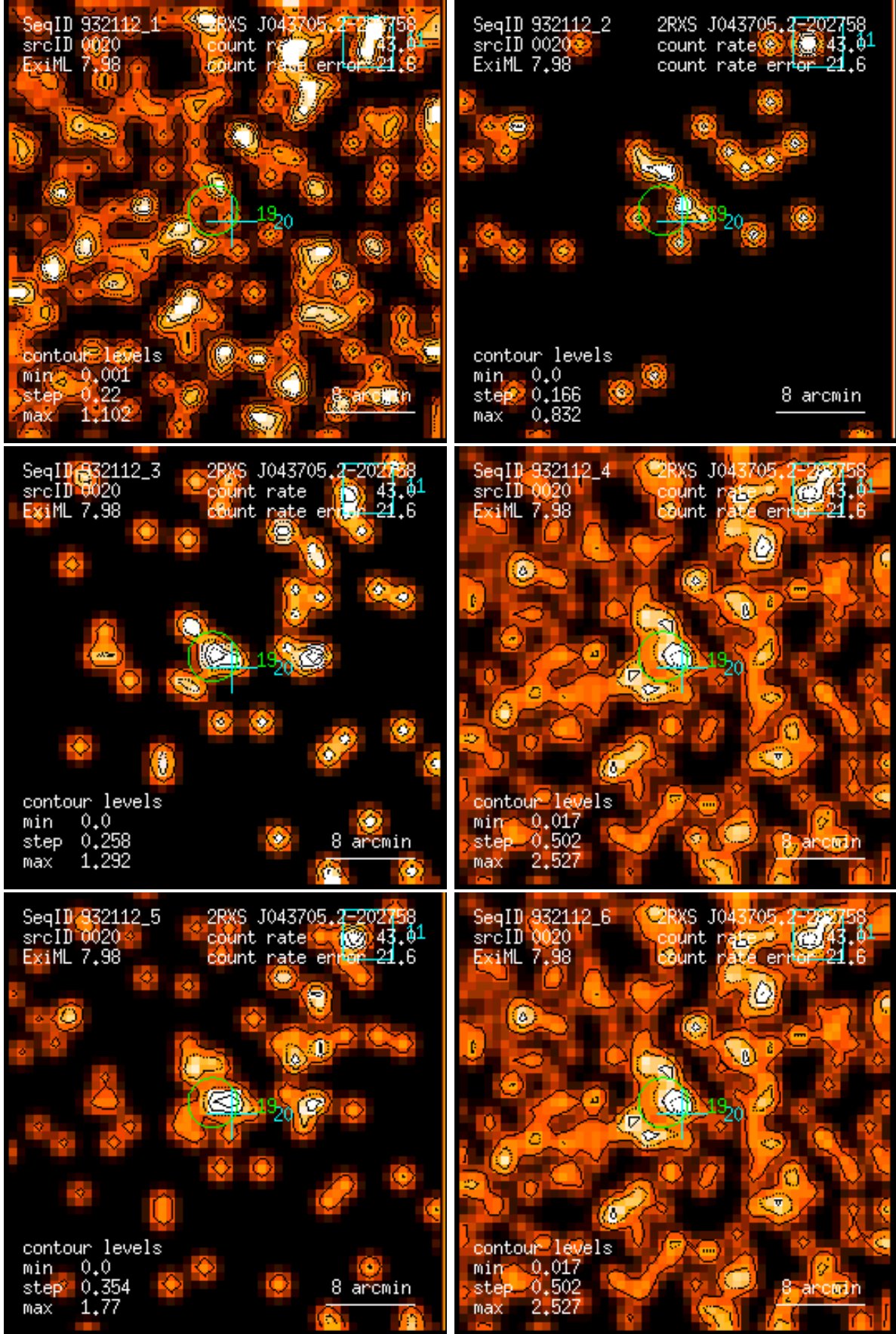
Figure 20: RASS 932112: detection 0020: band rate images, Gaussian filter: (1) PSPC channels 11 – 41, (2) 52 – 90, (3) 91 – 201, (4) 11 – 235, (5) 52 – 201, (6) 11 – 201. Broad band rates in counts/ks. Band rate contour levels in counts/ks/arcmin 2 .
