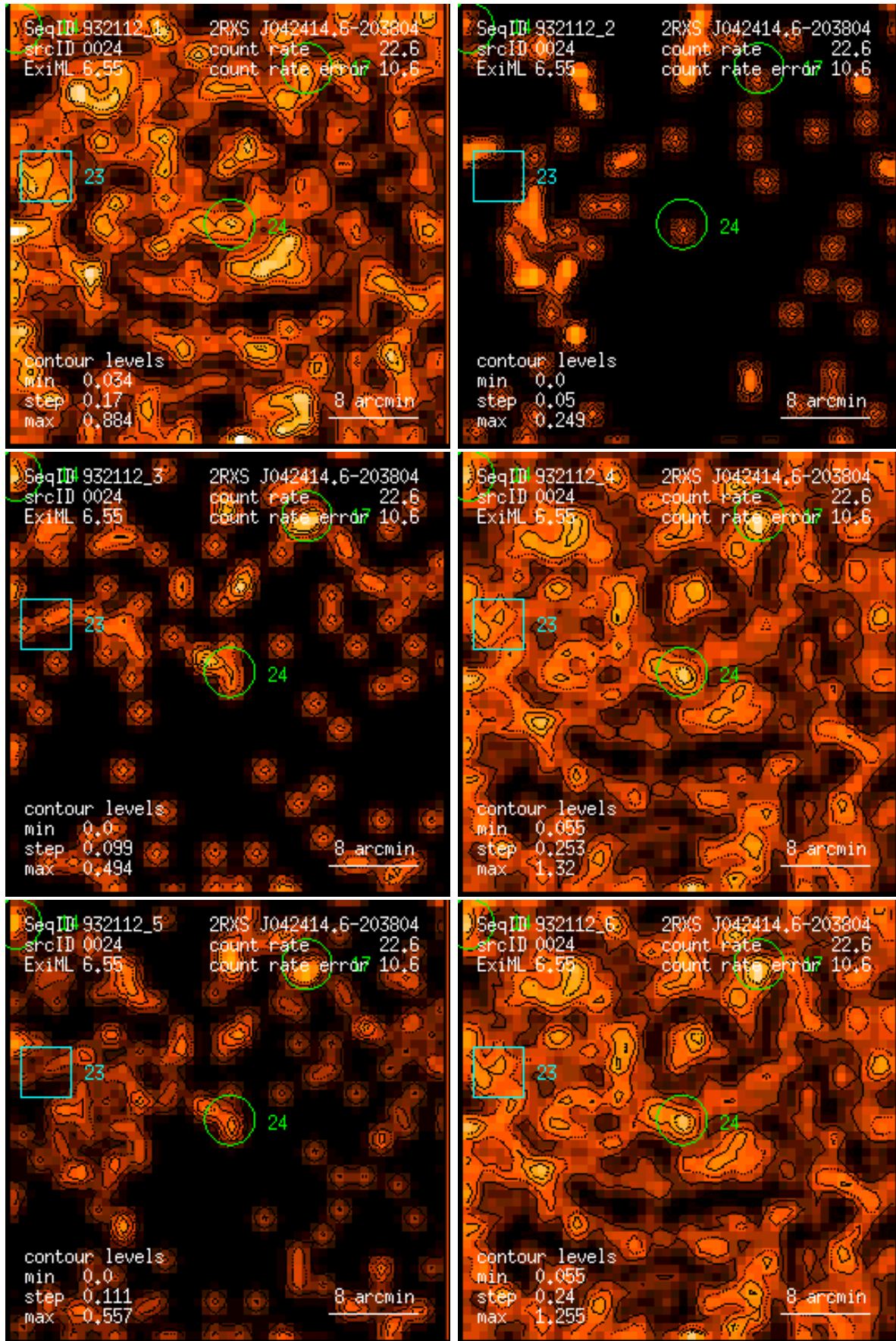
Figure 24: RASS 932112: detection 0024: band rate images, Gaussian filter: (1) PSPC channels 11 – 41, (2) 52 – 90, (3) 91 – 201, (4) 11 – 235, (5) 52 – 201, (6) 11 – 201. Broad band rates in counts/ks. Band rate contour levels in counts/ks/arcmin 2 .
