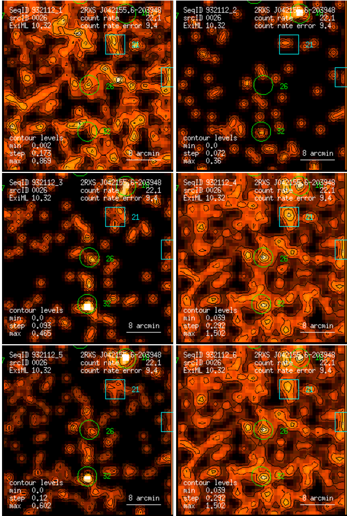
Figure 26: RASS 932112: detection 0026: band rate images, Gaussian filter: (1) PSPC channels 11 – 41, (2) 52 – 90, (3) 91 – 201, (4) 11 – 235, (5) 52 – 201, (6) 11 – 201. Broad band rates in counts/ks. Band rate contour levels in counts/ks/arcmin 2 .
