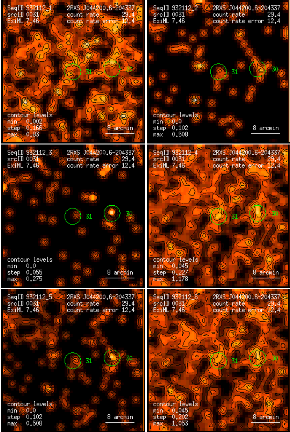
Figure 31: RASS 932112: detection 0031: band rate images, Gaussian filter: (1) PSPC channels 11 – 41, (2) 52 – 90, (3) 91 – 201, (4) 11 – 235, (5) 52 – 201, (6) 11 – 201. Broad band rates in counts/ks. Band rate contour levels in counts/ks/arcmin 2 .
