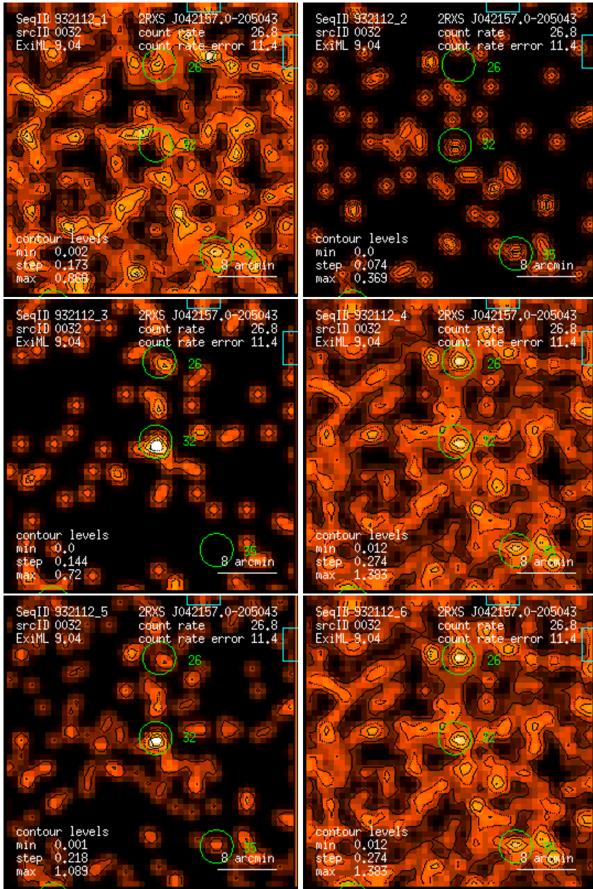
Figure 32: RASS 932112: detection 0032: band rate images, Gaussian filter: (1) PSPC channels 11 – 41, (2) 52 – 90, (3) 91 – 201, (4) 11 – 235, (5) 52 – 201, (6) 11 – 201. Broad band rates in counts/ks. Band rate contour levels in counts/ks/arcmin 2 .
