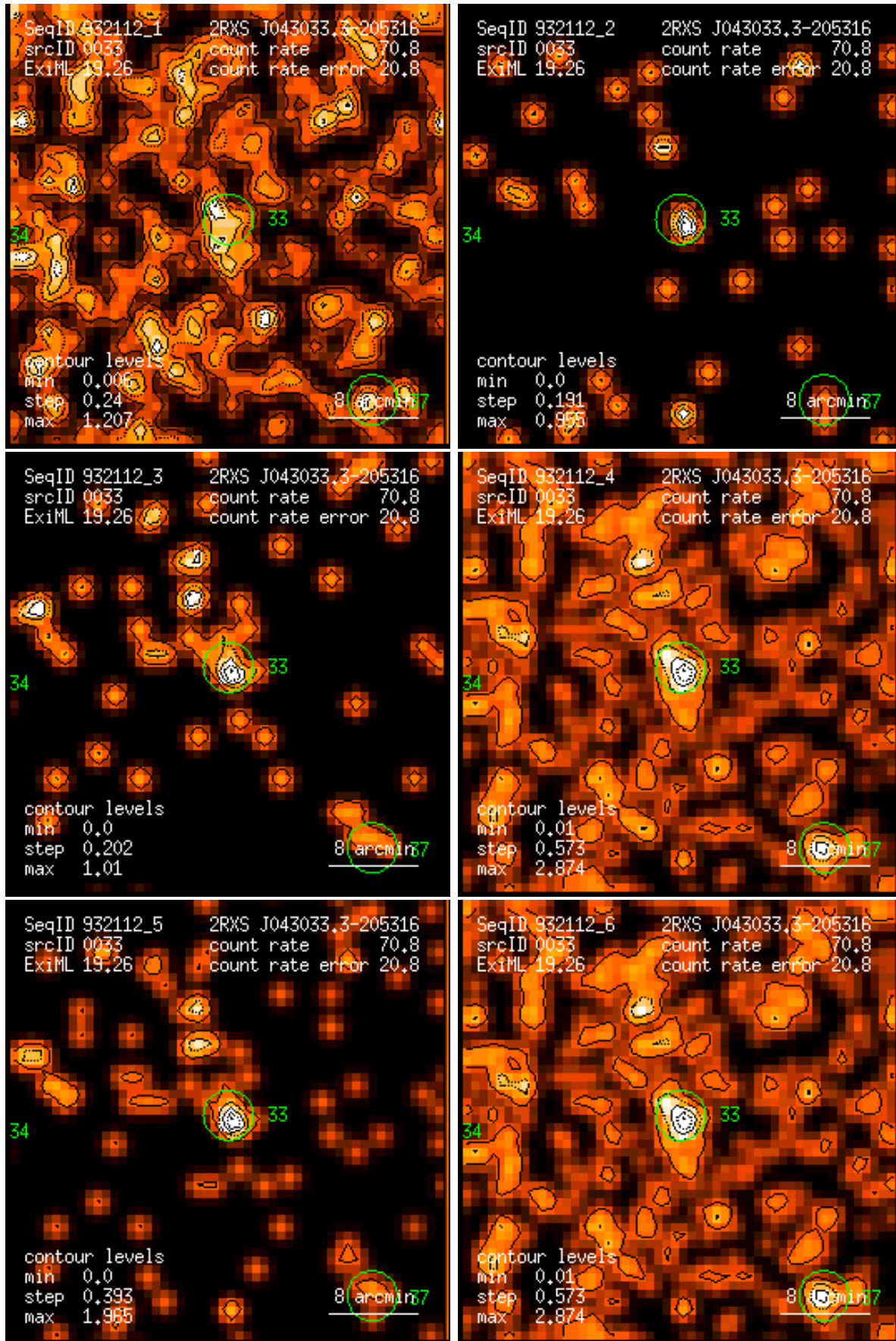
Figure 33: RASS 932112: detection 0033: band rate images, Gaussian filter: (1) PSPC channels 11 – 41, (2) 52 – 90, (3) 91 – 201, (4) 11 – 235, (5) 52 – 201, (6) 11 – 201. Broad band rates in counts/ks. Band rate contour levels in counts/ks/arcmin 2 .
