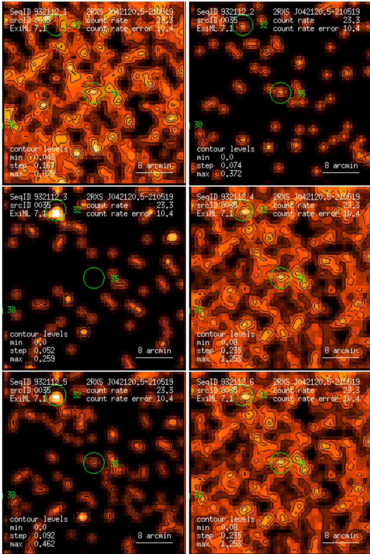
Figure 35: RASS 932112: detection 0035: band rate images, Gaussian filter: (1) PSPC channels 11 – 41, (2) 52 – 90, (3) 91 – 201, (4) 11 – 235, (5) 52 – 201, (6) 11 – 201. Broad band rates in counts/ks. Band rate contour levels in counts/ks/arcmin 2 .
