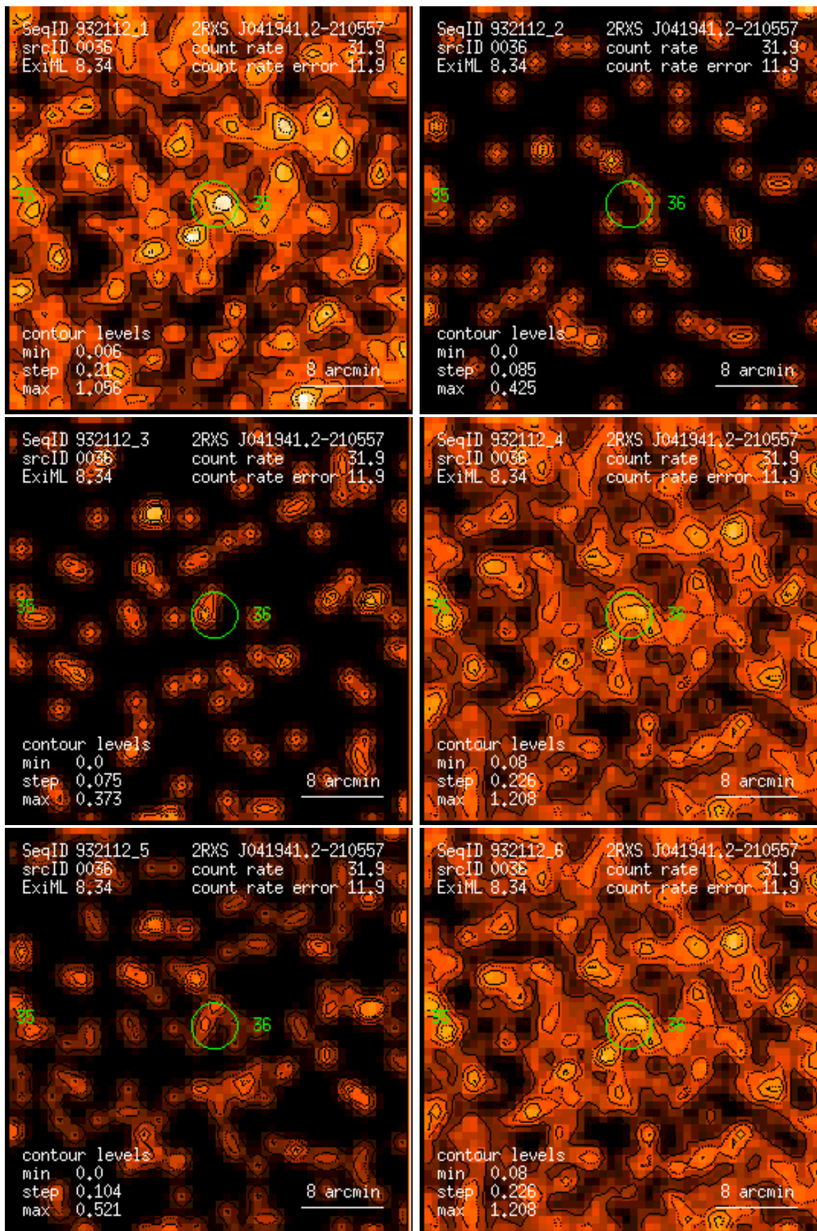
Figure 36: RASS 932112: detection 0036: band rate images, Gaussian filter: (1) PSPC channels 11 – 41, (2) 52 – 90, (3) 91 – 201, (4) 11 – 235, (5) 52 – 201, (6) 11 – 201. Broad band rates in counts/ks. Band rate contour levels in counts/ks/arcmin 2 .
