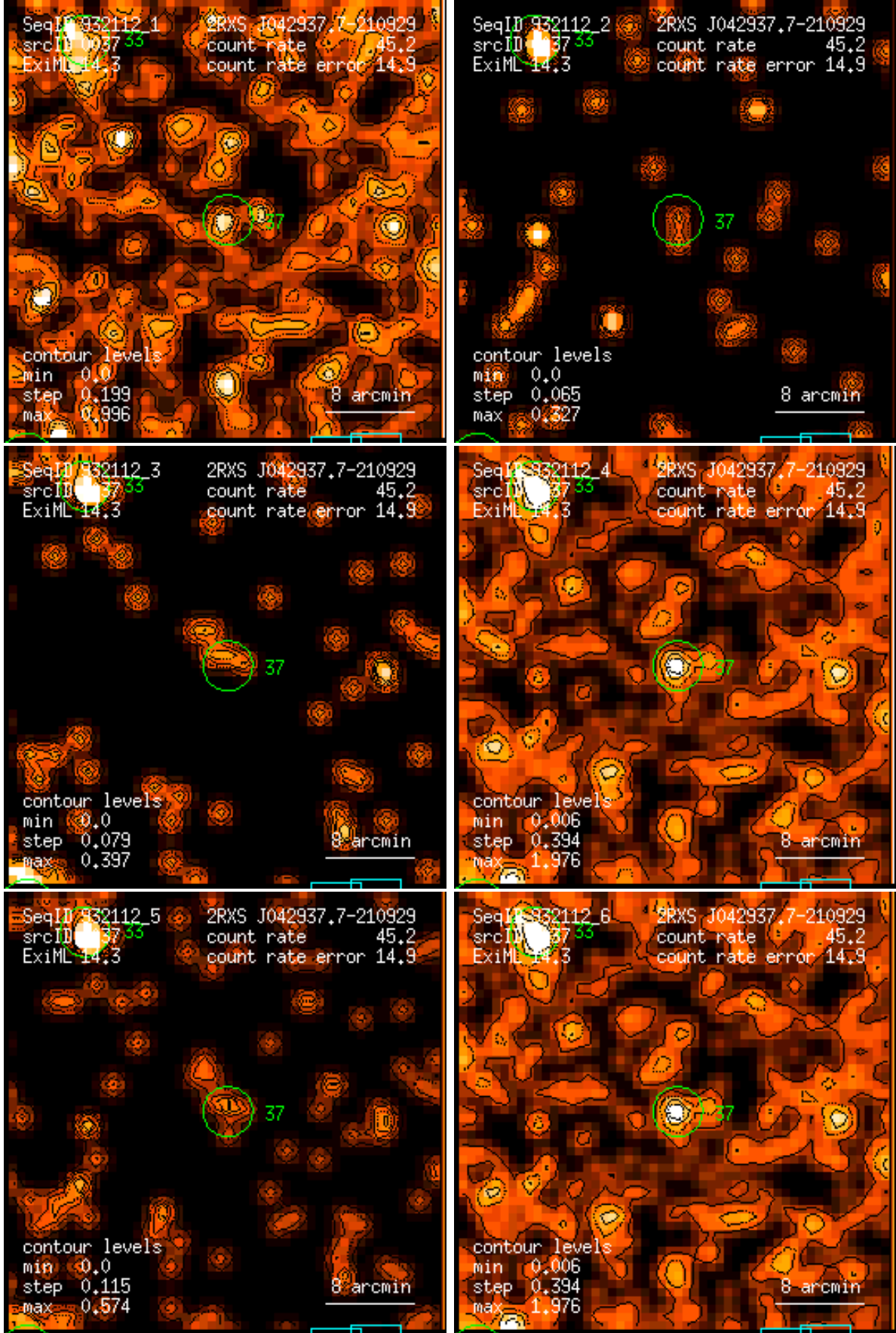
Figure 37: RASS 932112: detection 0037: band rate images, Gaussian filter: (1) PSPC channels 11 – 41, (2) 52 – 90, (3) 91 – 201, (4) 11 – 235, (5) 52 – 201, (6) 11 – 201. Broad band rates in counts/ks. Band rate contour levels in counts/ks/arcmin 2 .
