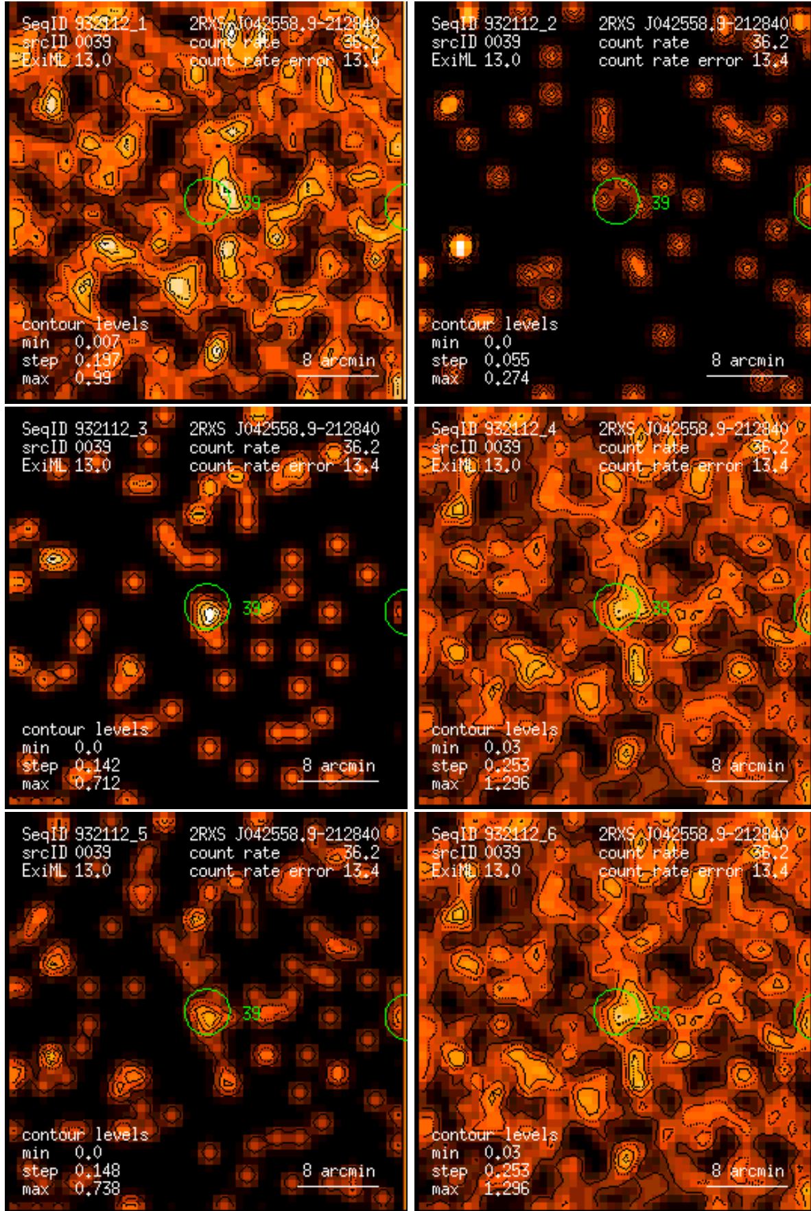
Figure 39: RASS 932112: detection 0039: band rate images, Gaussian filter: (1) PSPC channels 11 – 41, (2) 52 – 90, (3) 91 – 201, (4) 11 – 235, (5) 52 – 201, (6) 11 – 201. Broad band rates in counts/ks. Band rate contour levels in counts/ks/arcmin 2 .
