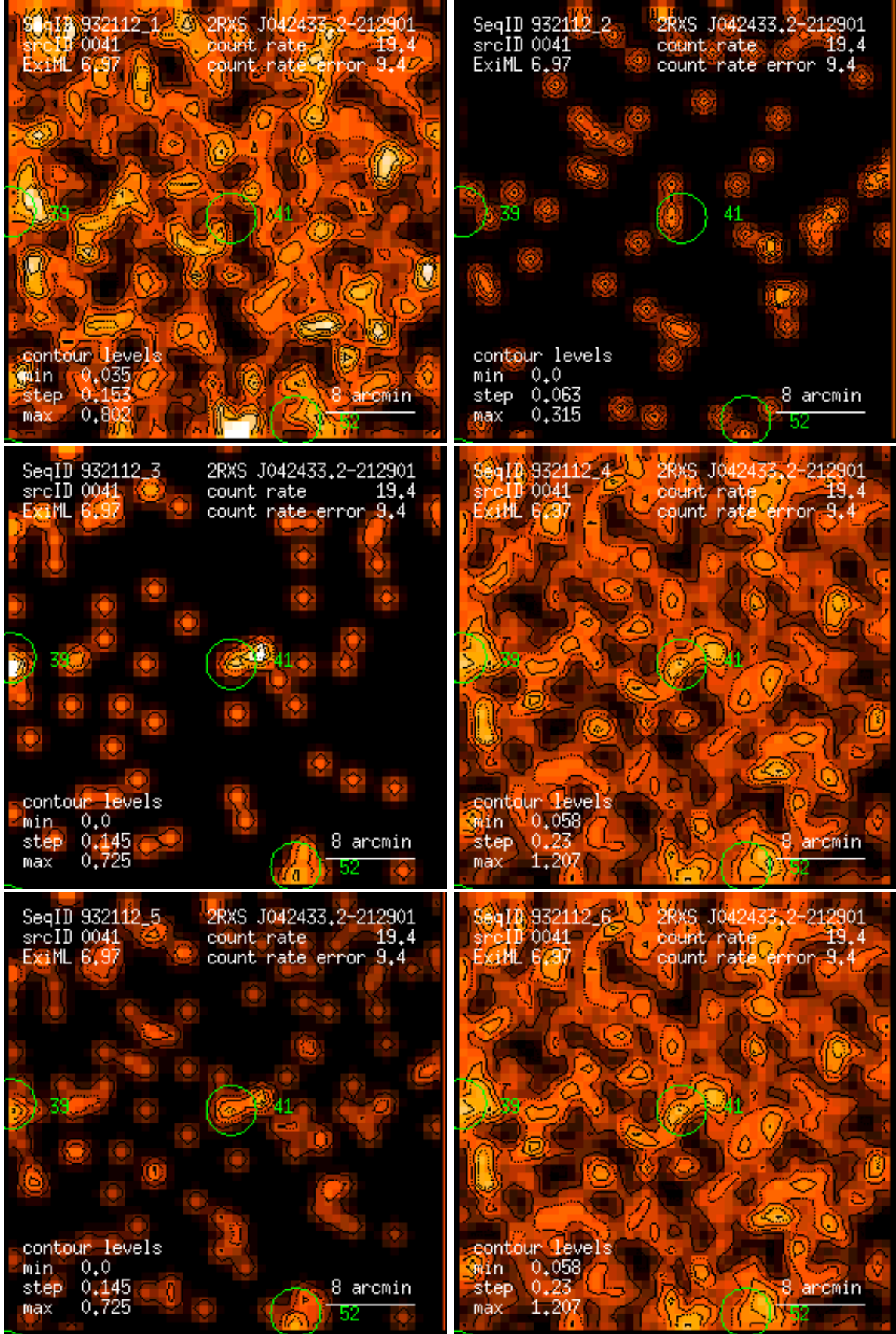
Figure 41: RASS 932112: detection 0041: band rate images, Gaussian filter: (1) PSPC channels 11 – 41, (2) 52 – 90, (3) 91 – 201, (4) 11 – 235, (5) 52 – 201, (6) 11 – 201. Broad band rates in counts/ks. Band rate contour levels in counts/ks/arcmin 2 .
