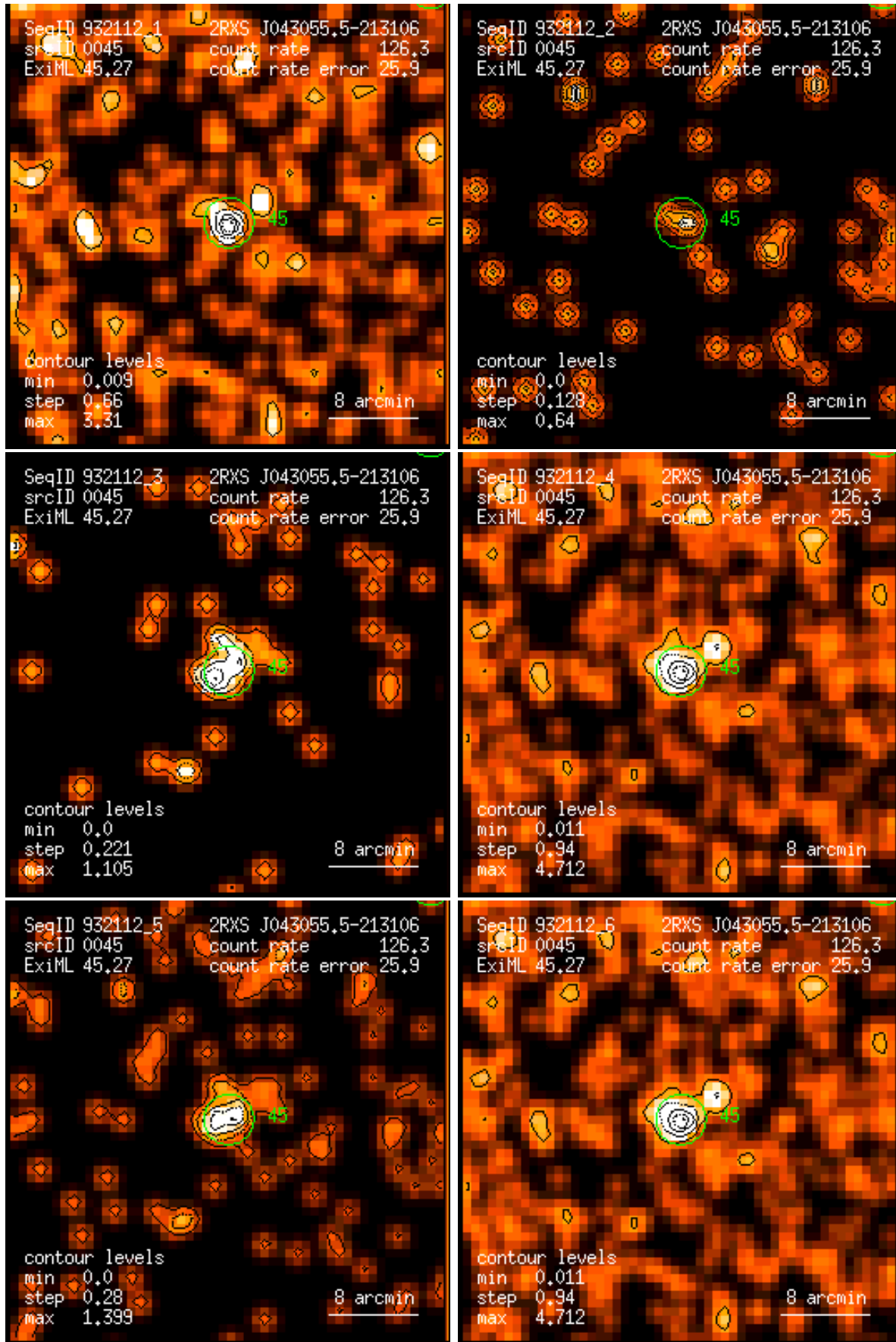
Figure 45: RASS 932112: detection 0045: band rate images, Gaussian filter: (1) PSPC channels 11 – 41, (2) 52 – 90, (3) 91 – 201, (4) 11 – 235, (5) 52 – 201, (6) 11 – 201. Broad band rates in counts/ks. Band rate contour levels in counts/ks/arcmin 2 .
