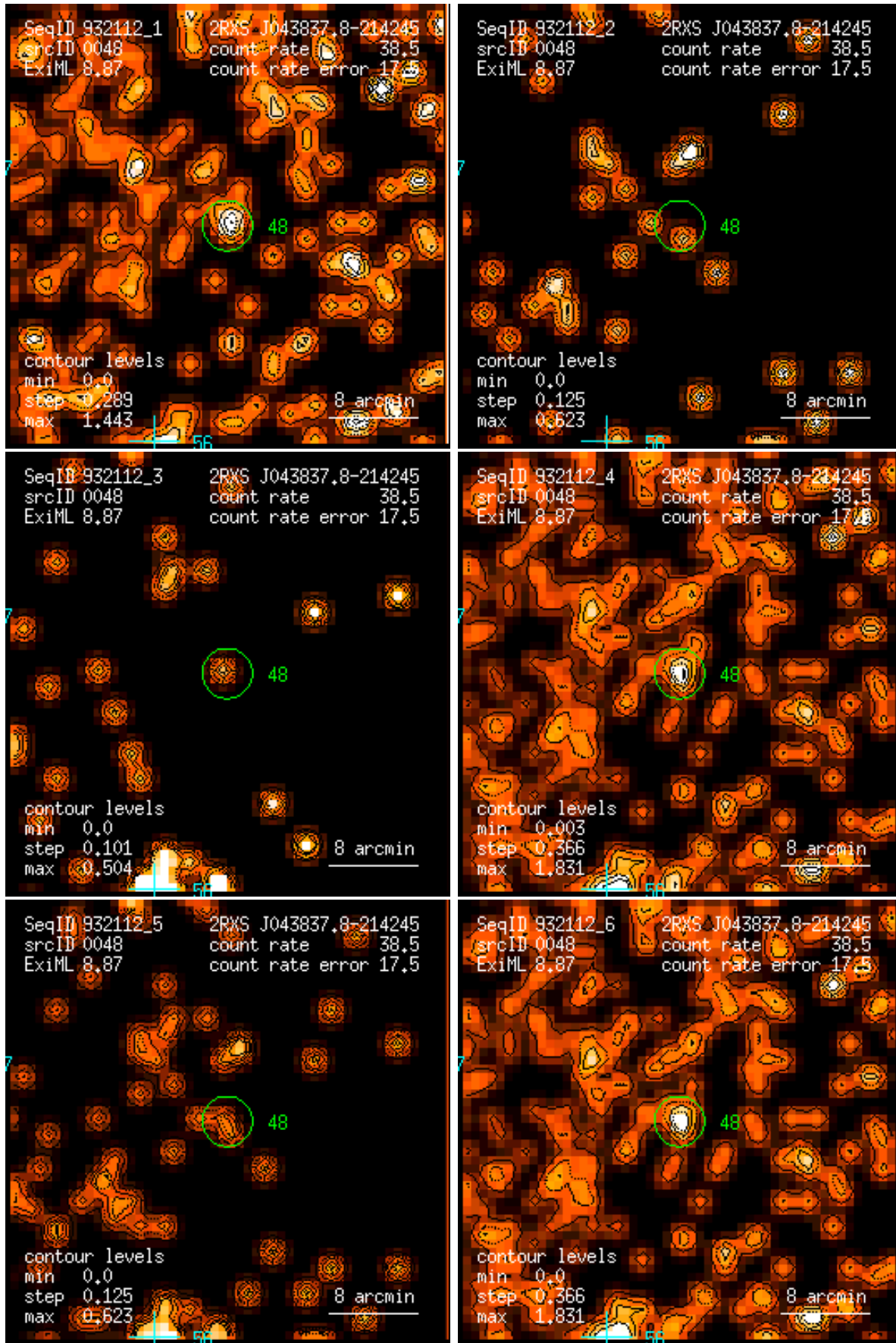
Figure 48: RASS 932112: detection 0048: band rate images, Gaussian filter: (1) PSPC channels 11 – 41, (2) 52 – 90, (3) 91 – 201, (4) 11 – 235, (5) 52 – 201, (6) 11 – 201. Broad band rates in counts/ks. Band rate contour levels in counts/ks/arcmin 2 .
