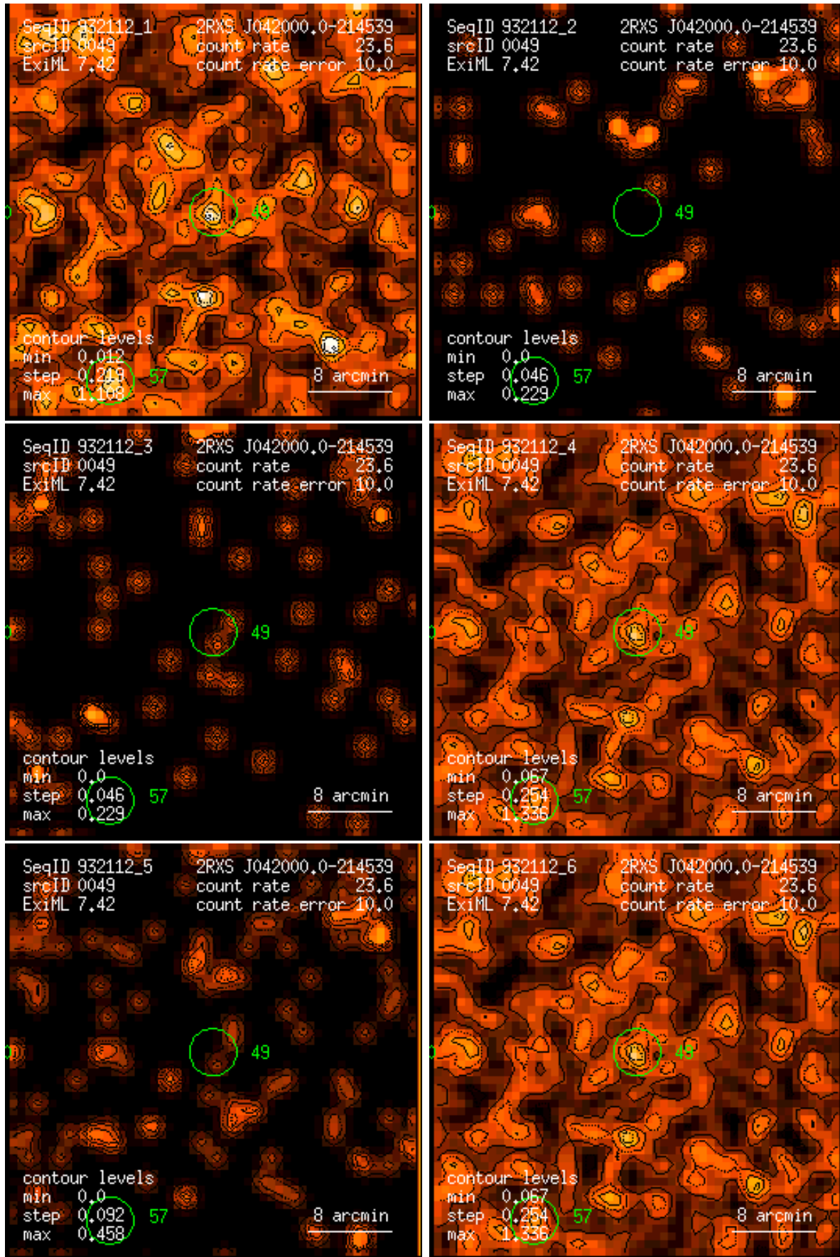
Figure 49: RASS 932112: detection 0049: band rate images, Gaussian filter: (1) PSPC channels 11 – 41, (2) 52 – 90, (3) 91 – 201, (4) 11 – 235, (5) 52 – 201, (6) 11 – 201. Broad band rates in counts/ks. Band rate contour levels in counts/ks/arcmin 2 .
