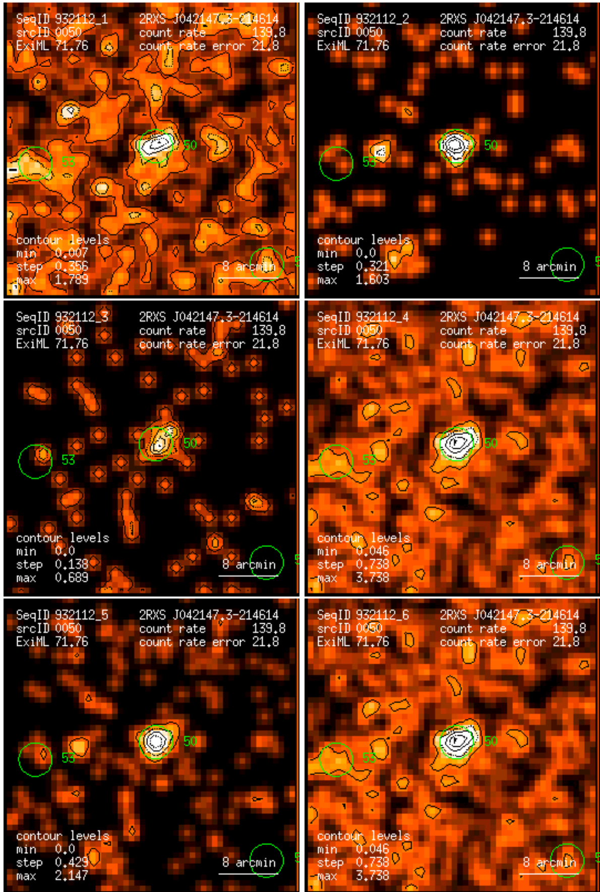
Figure 50: RASS 932112: detection 0050: band rate images, Gaussian filter: (1) PSPC channels 11 – 41, (2) 52 – 90, (3) 91 – 201, (4) 11 – 235, (5) 52 – 201, (6) 11 – 201. Broad band rates in counts/ks. Band rate contour levels in counts/ks/arcmin 2 .
