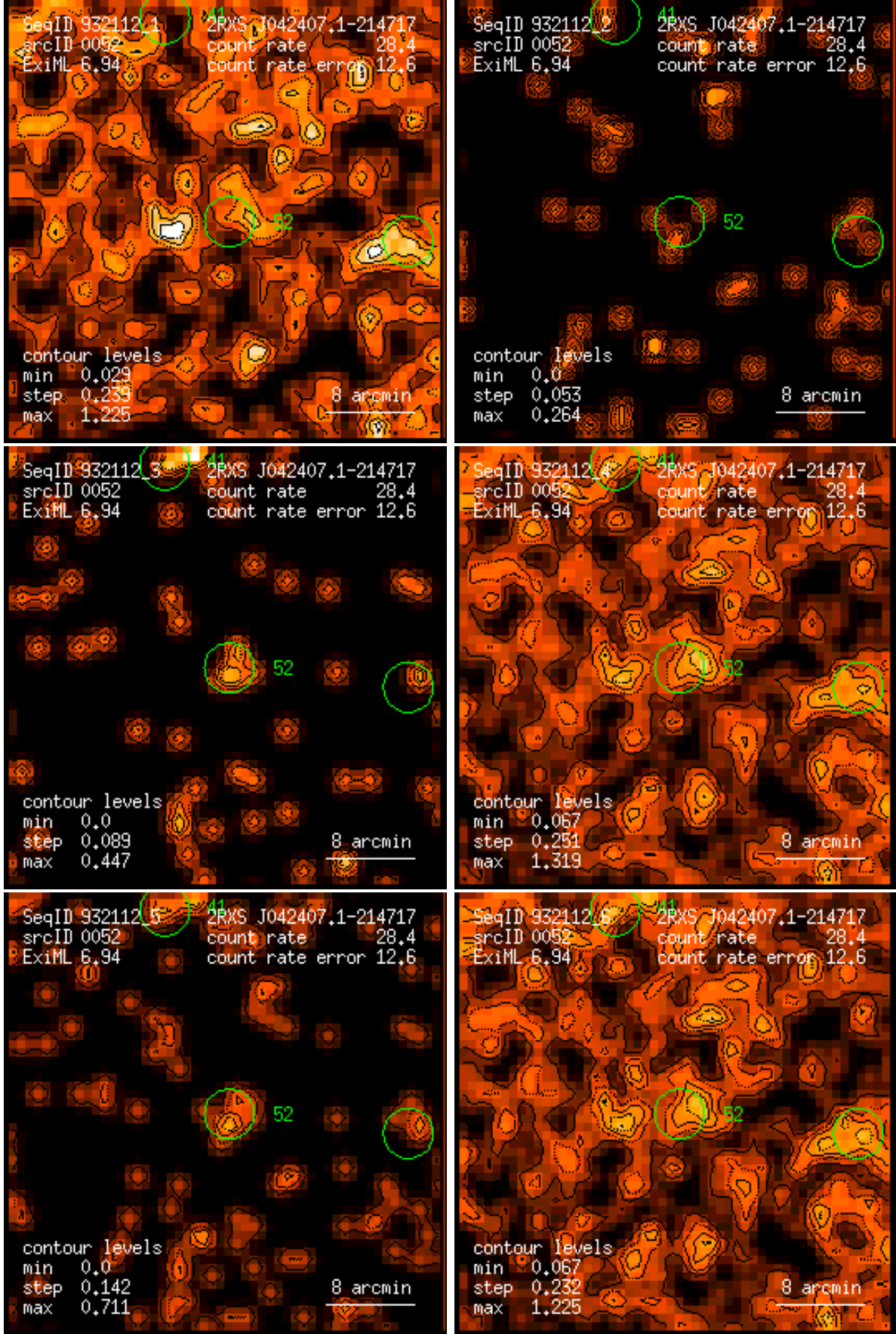
Figure 52: RASS 932112: detection 0052: band rate images, Gaussian filter: (1) PSPC channels 11 – 41, (2) 52 – 90, (3) 91 – 201, (4) 11 – 235, (5) 52 – 201, (6) 11 – 201. Broad band rates in counts/ks. Band rate contour levels in counts/ks/arcmin 2 .
