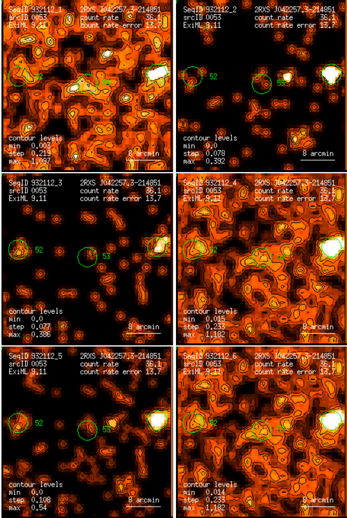
Figure 53: RASS 932112: detection 0053: band rate images, Gaussian filter: (1) PSPC channels 11 – 41, (2) 52 – 90, (3) 91 – 201, (4) 11 – 235, (5) 52 – 201, (6) 11 – 201. Broad band rates in counts/ks. Band rate contour levels in counts/ks/arcmin 2 .
