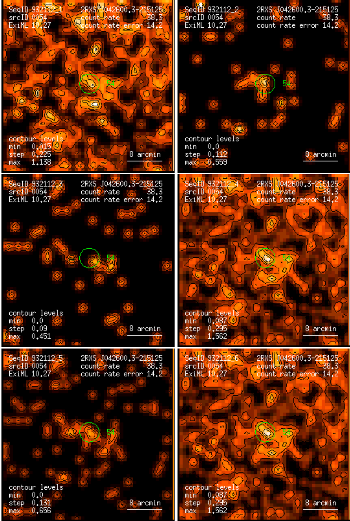
Figure 54: RASS 932112: detection 0054: band rate images, Gaussian filter: (1) PSPC channels 11 – 41, (2) 52 – 90, (3) 91 – 201, (4) 11 – 235, (5) 52 – 201, (6) 11 – 201. Broad band rates in counts/ks. Band rate contour levels in counts/ks/arcmin 2 .
