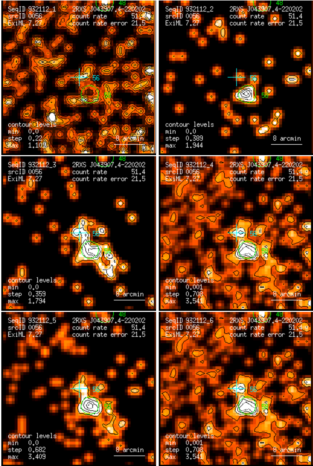
Figure 56: RASS 932112: detection 0056: band rate images, Gaussian filter: (1) PSPC channels 11 – 41, (2) 52 – 90, (3) 91 – 201, (4) 11 – 235, (5) 52 – 201, (6) 11 – 201. Broad band rates in counts/ks. Band rate contour levels in counts/ks/arcmin 2 .
