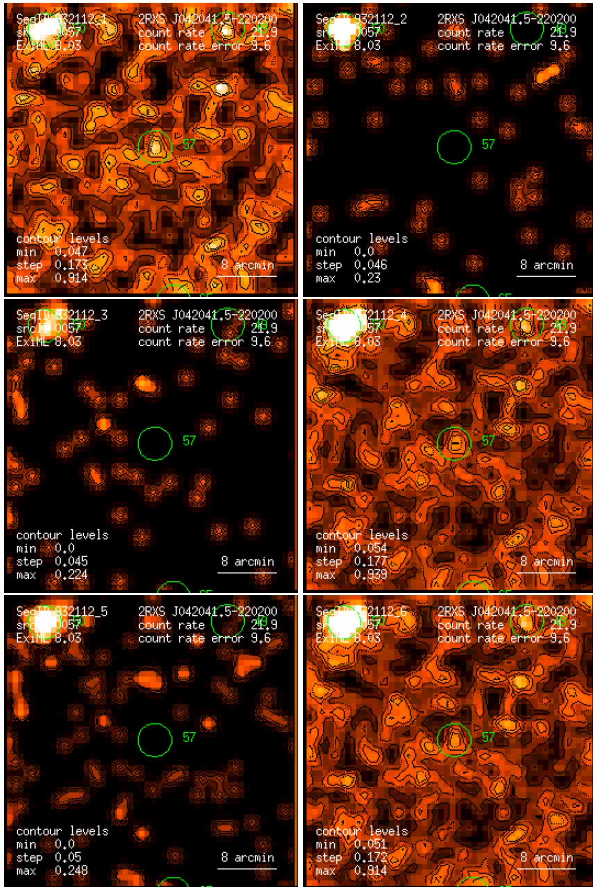
Figure 57: RASS 932112: detection 0057: band rate images, Gaussian filter: (1) PSPC channels 11 – 41, (2) 52 – 90, (3) 91 – 201, (4) 11 – 235, (5) 52 – 201, (6) 11 – 201. Broad band rates in counts/ks. Band rate contour levels in counts/ks/arcmin 2 .
