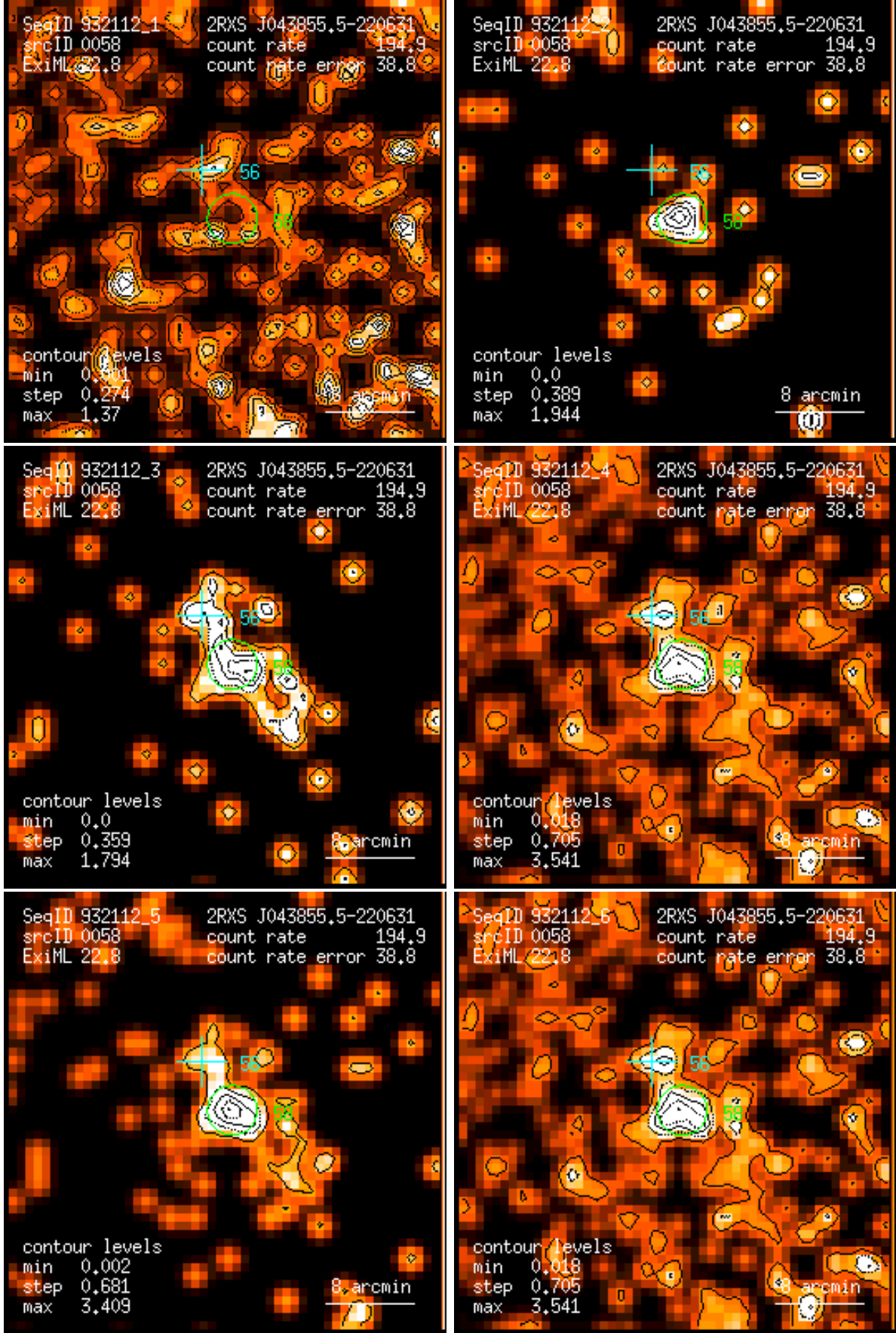
Figure 58: RASS 932112: detection 0058: band rate images, Gaussian filter: (1) PSPC channels 11 – 41, (2) 52 – 90, (3) 91 – 201, (4) 11 – 235, (5) 52 – 201, (6) 11 – 201. Broad band rates in counts/ks. Band rate contour levels in counts/ks/arcmin 2 .
