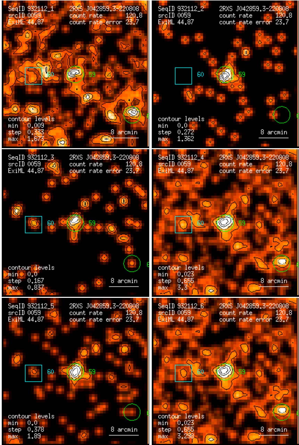
Figure 59: RASS 932112: detection 0059: band rate images, Gaussian filter: (1) PSPC channels 11 – 41, (2) 52 – 90, (3) 91 – 201, (4) 11 – 235, (5) 52 – 201, (6) 11 – 201. Broad band rates in counts/ks. Band rate contour levels in counts/ks/arcmin 2 .
