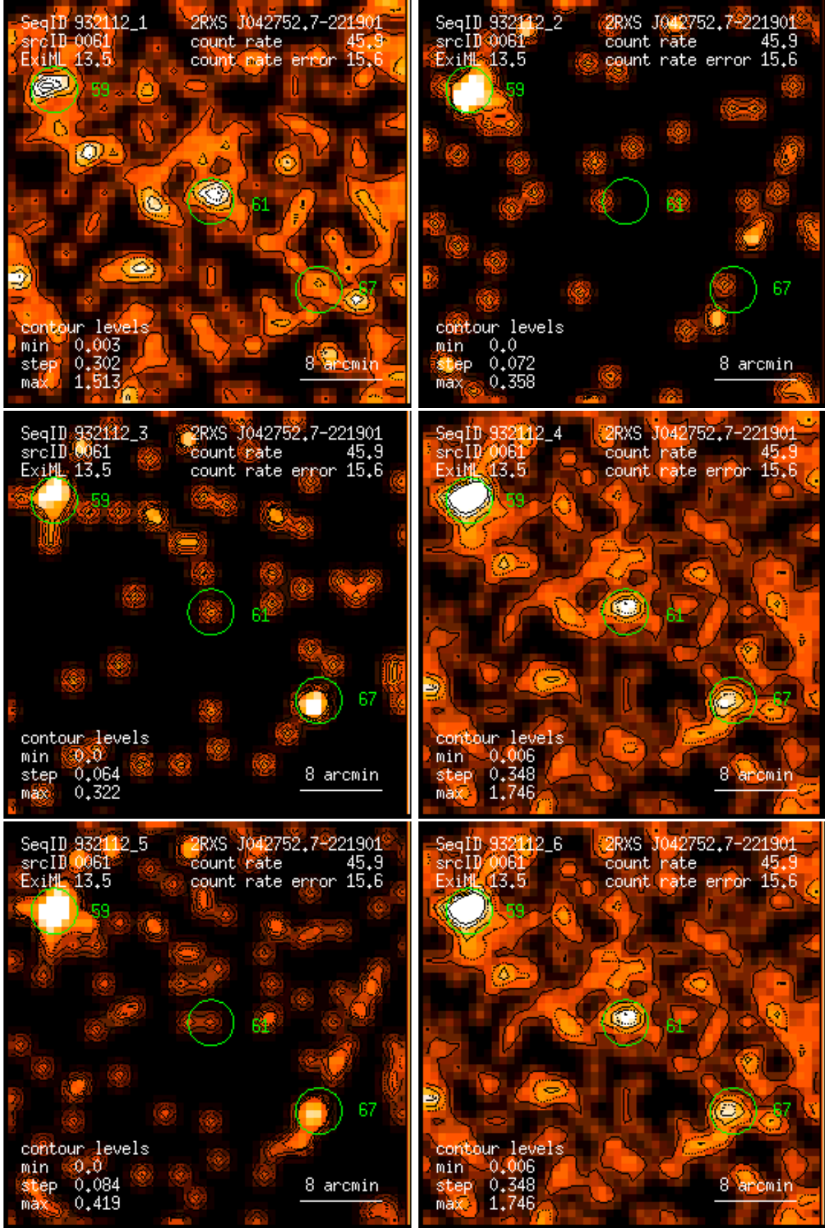
Figure 61: RASS 932112: detection 0061: band rate images, Gaussian filter: (1) PSPC channels 11 – 41, (2) 52 – 90, (3) 91 – 201, (4) 11 – 235, (5) 52 – 201, (6) 11 – 201. Broad band rates in counts/ks. Band rate contour levels in counts/ks/arcmin 2 .
