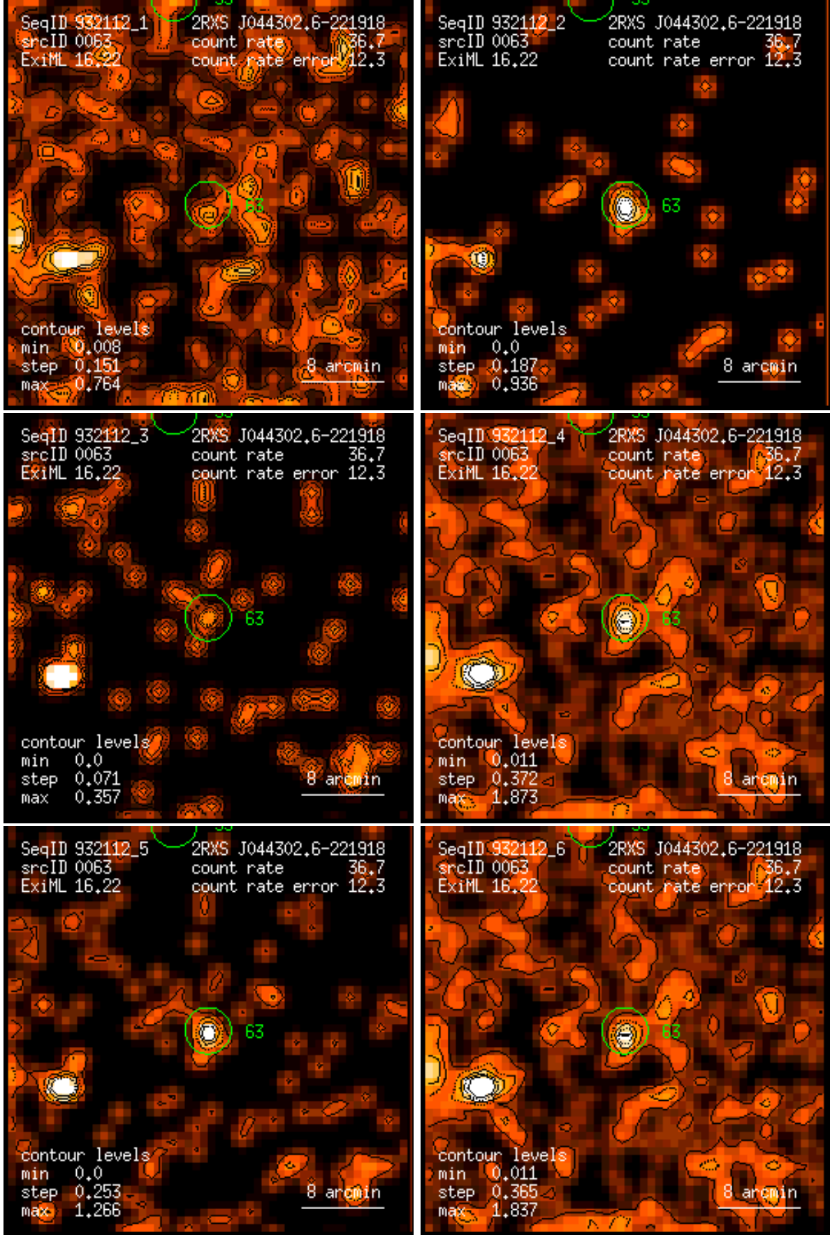
Figure 63: RASS 932112: detection 0063: band rate images, Gaussian filter: (1) PSPC channels 11 – 41, (2) 52 – 90, (3) 91 – 201, (4) 11 – 235, (5) 52 – 201, (6) 11 – 201. Broad band rates in counts/ks. Band rate contour levels in counts/ks/arcmin 2 .
