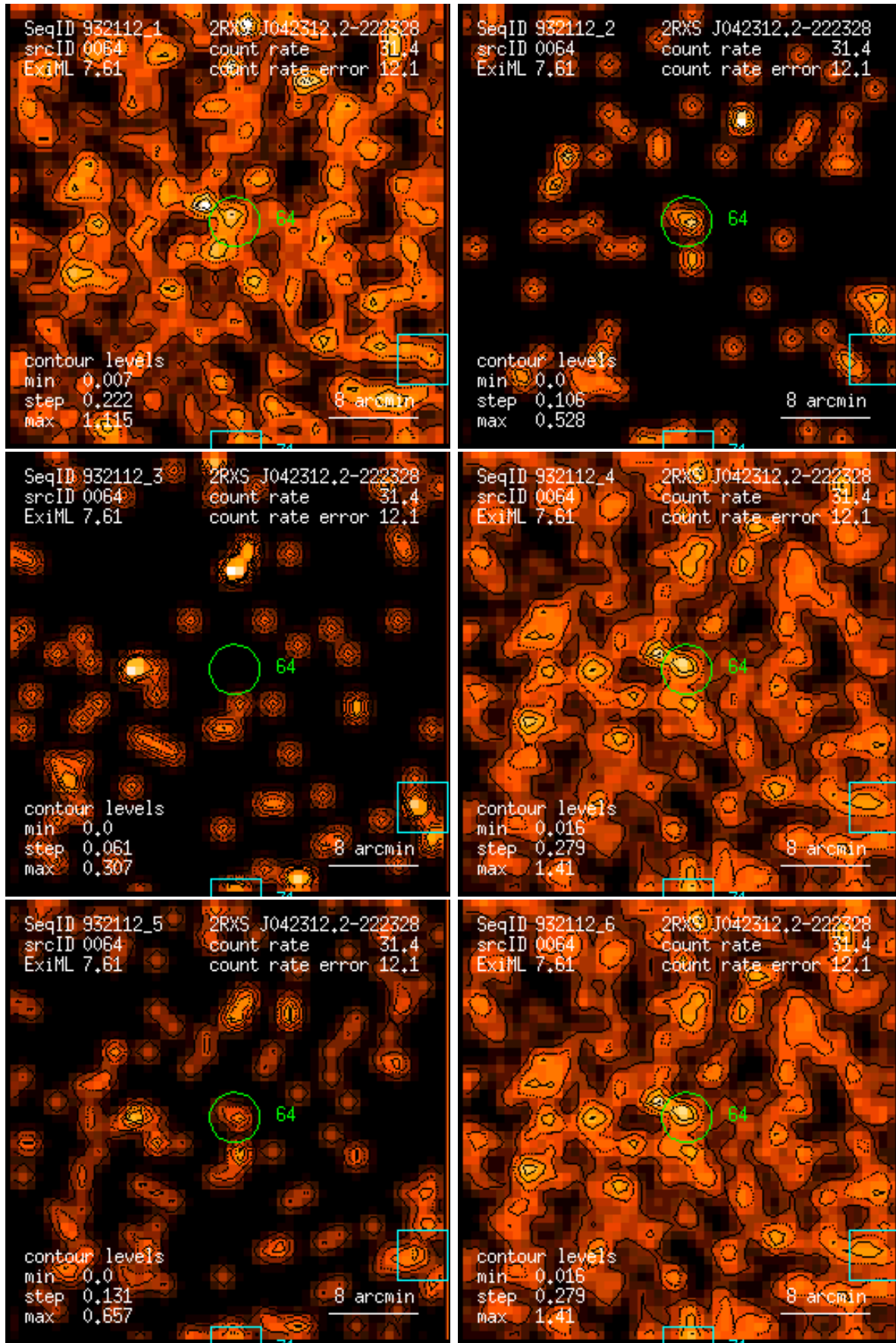
Figure 64: RASS 932112: detection 0064: band rate images, Gaussian filter: (1) PSPC channels 11 – 41, (2) 52 – 90, (3) 91 – 201, (4) 11 – 235, (5) 52 – 201, (6) 11 – 201. Broad band rates in counts/ks. Band rate contour levels in counts/ks/arcmin 2 .
