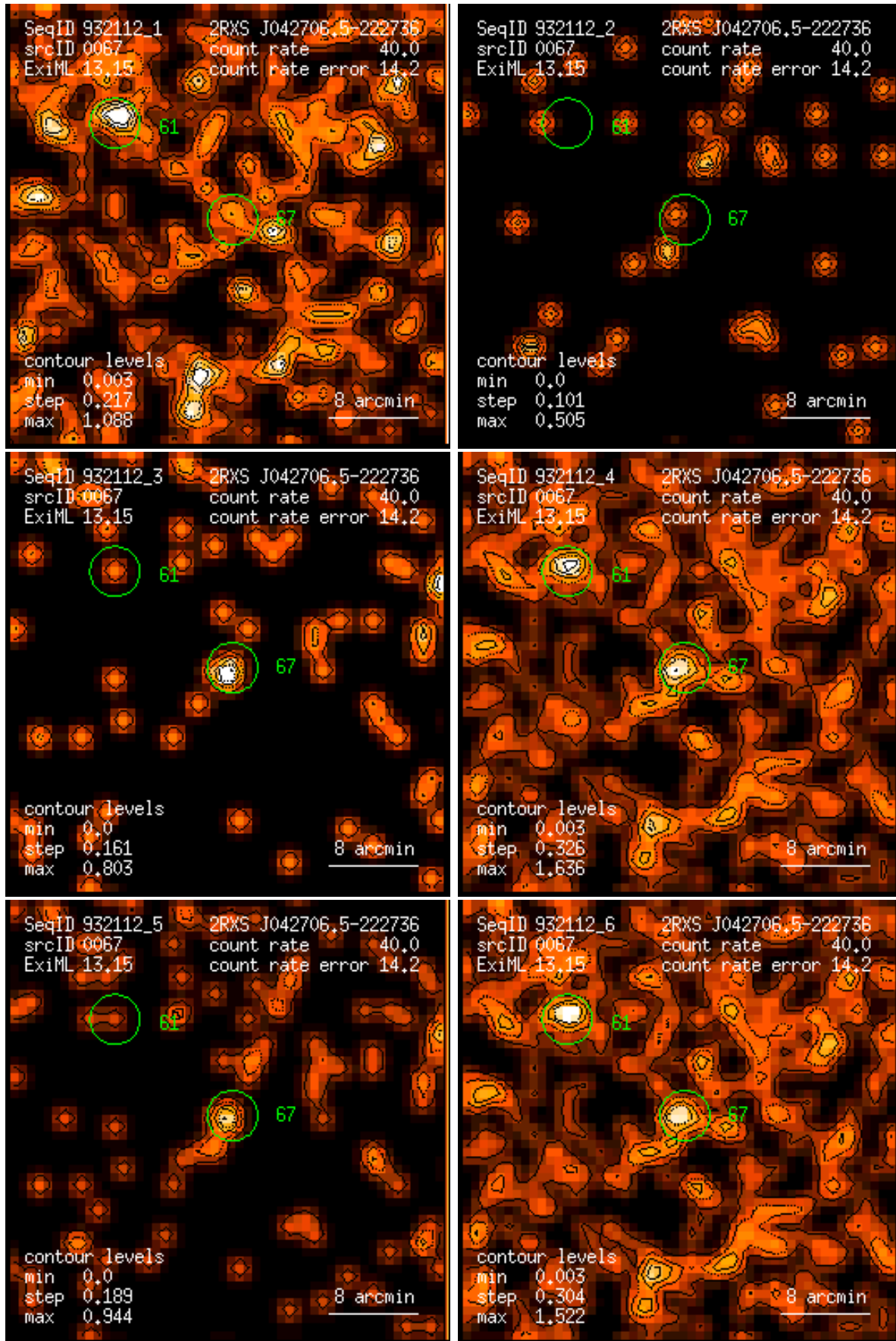
Figure 67: RASS 932112: detection 0067: band rate images, Gaussian filter: (1) PSPC channels 11 – 41, (2) 52 – 90, (3) 91 – 201, (4) 11 – 235, (5) 52 – 201, (6) 11 – 201. Broad band rates in counts/ks. Band rate contour levels in counts/ks/arcmin 2 .
