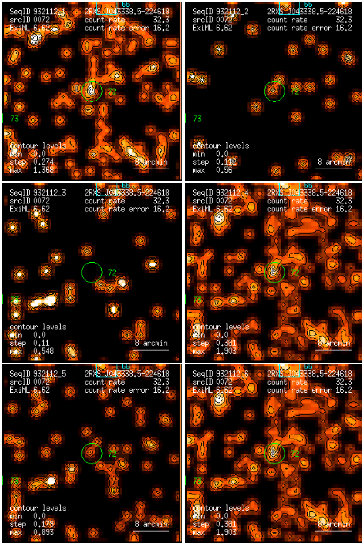
Figure 72: RASS 932112: detection 0072: band rate images, Gaussian filter: (1) PSPC channels 11 – 41, (2) 52 – 90, (3) 91 – 201, (4) 11 – 235, (5) 52 – 201, (6) 11 – 201. Broad band rates in counts/ks. Band rate contour levels in counts/ks/arcmin 2 .
