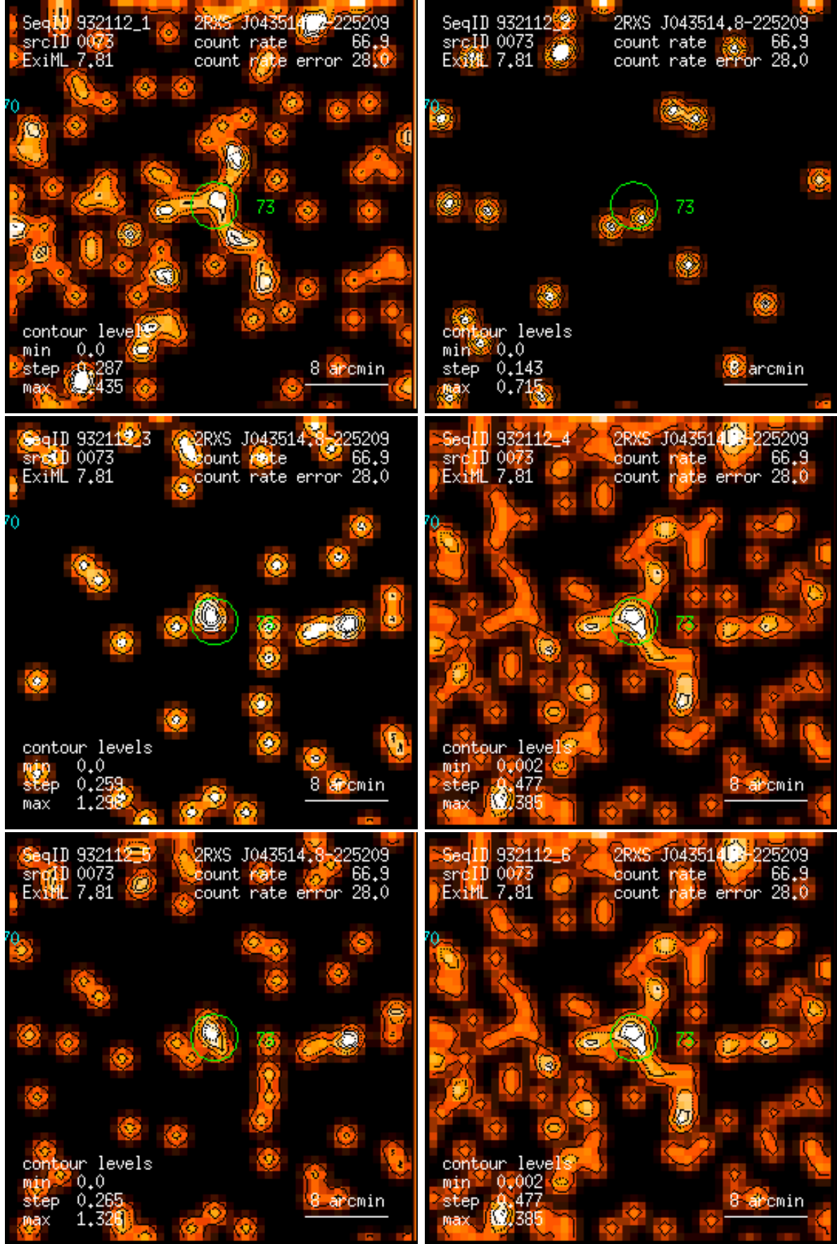
Figure 73: RASS 932112: detection 0073: band rate images, Gaussian filter: (1) PSPC channels 11 – 41, (2) 52 – 90, (3) 91 – 201, (4) 11 – 235, (5) 52 – 201, (6) 11 – 201. Broad band rates in counts/ks. Band rate contour levels in counts/ks/arcmin 2 .
