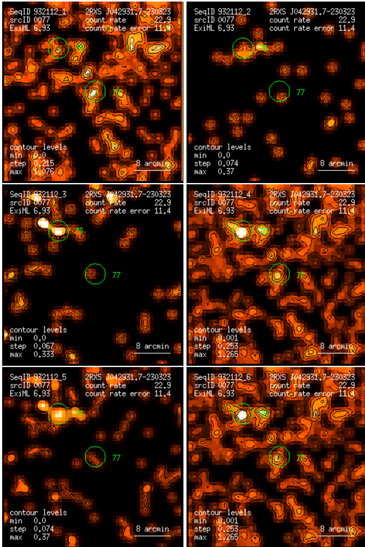
Figure 77: RASS 932112: detection 0077: band rate images, Gaussian filter: (1) PSPC channels 11 – 41, (2) 52 – 90, (3) 91 – 201, (4) 11 – 235, (5) 52 – 201, (6) 11 – 201. Broad band rates in counts/ks. Band rate contour levels in counts/ks/arcmin 2 .
