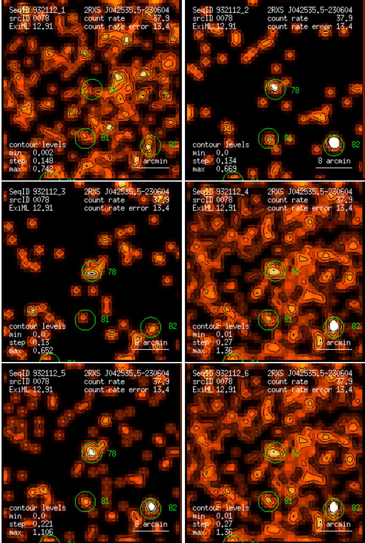
Figure 78: RASS 932112: detection 0078: band rate images, Gaussian filter: (1) PSPC channels 11 – 41, (2) 52 – 90, (3) 91 – 201, (4) 11 – 235, (5) 52 – 201, (6) 11 – 201. Broad band rates in counts/ks. Band rate contour levels in counts/ks/arcmin 2 .
