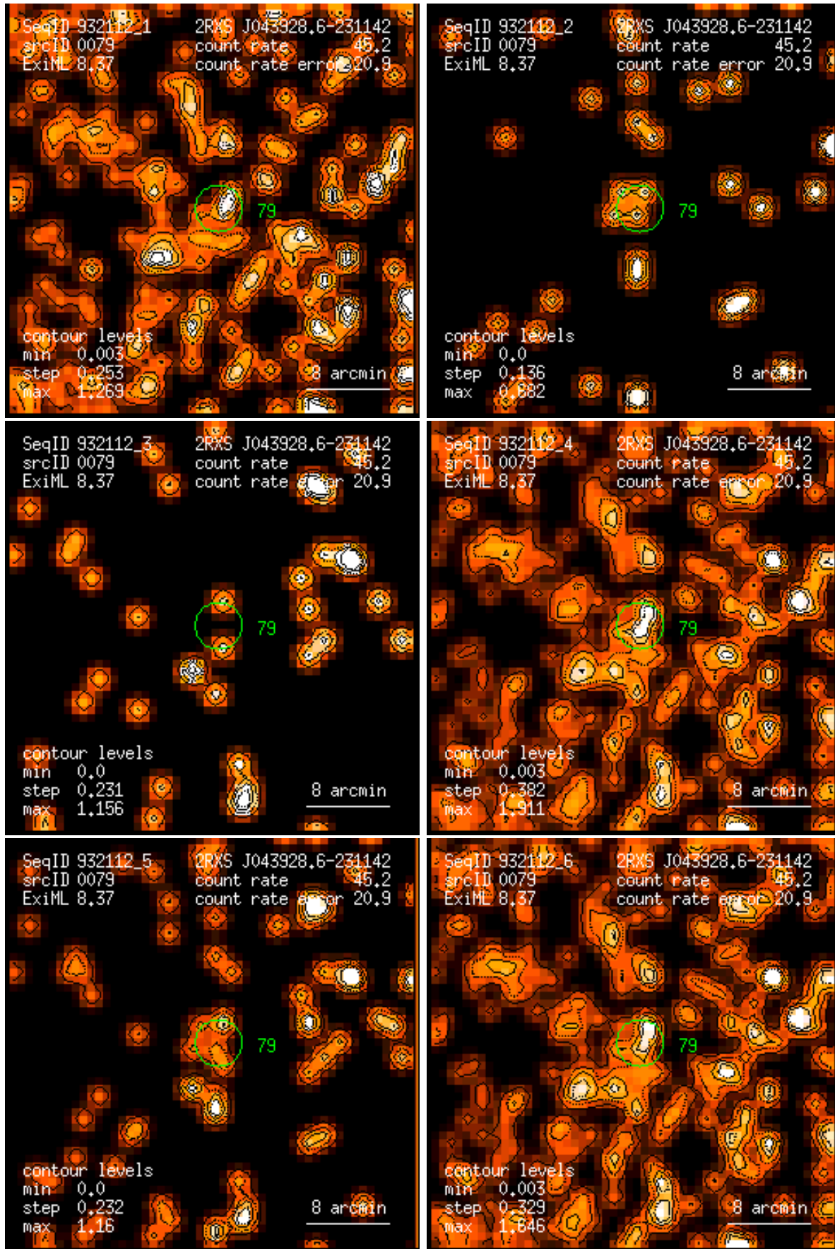
Figure 79: RASS 932112: detection 0079: band rate images, Gaussian filter: (1) PSPC channels 11 – 41, (2) 52 – 90, (3) 91 – 201, (4) 11 – 235, (5) 52 – 201, (6) 11 – 201. Broad band rates in counts/ks. Band rate contour levels in counts/ks/arcmin 2 .
