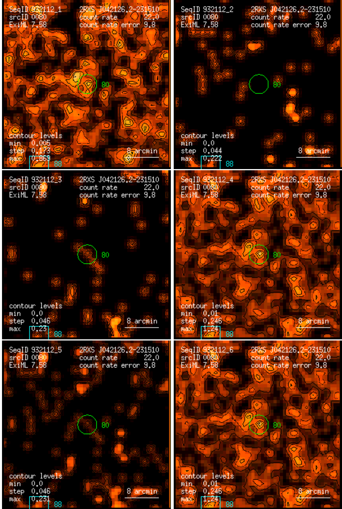
Figure 80: RASS 932112: detection 0080: band rate images, Gaussian filter: (1) PSPC channels 11 – 41, (2) 52 – 90, (3) 91 – 201, (4) 11 – 235, (5) 52 – 201, (6) 11 – 201. Broad band rates in counts/ks. Band rate contour levels in counts/ks/arcmin 2 .
