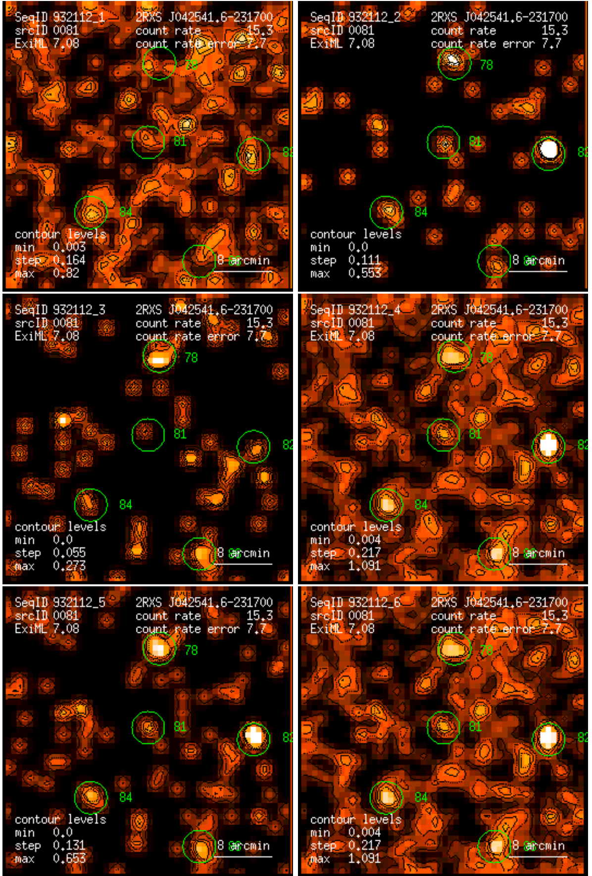
Figure 81: RASS 932112: detection 0081: band rate images, Gaussian filter: (1) PSPC channels 11 – 41, (2) 52 – 90, (3) 91 – 201, (4) 11 – 235, (5) 52 – 201, (6) 11 – 201. Broad band rates in counts/ks. Band rate contour levels in counts/ks/arcmin 2 .
