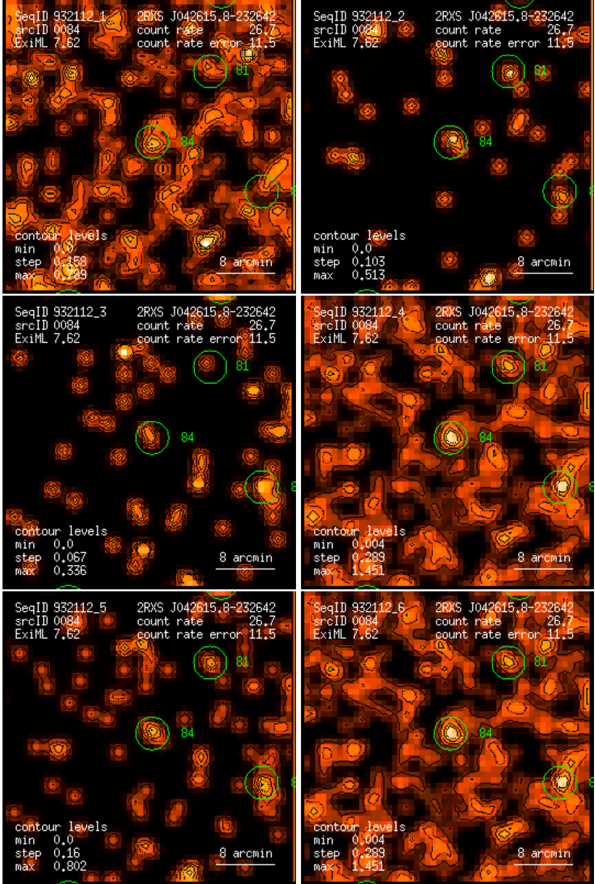
Figure 84: RASS 932112: detection 0084: band rate images, Gaussian filter: (1) PSPC channels 11 – 41, (2) 52 – 90, (3) 91 – 201, (4) 11 – 235, (5) 52 – 201, (6) 11 – 201. Broad band rates in counts/ks. Band rate contour levels in counts/ks/arcmin 2 .
