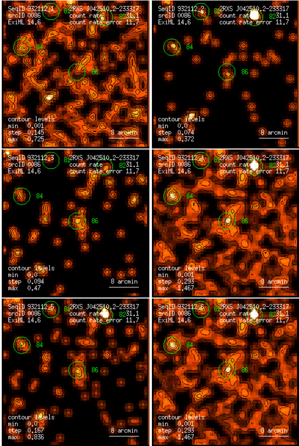
Figure 86: RASS 932112: detection 0086: band rate images, Gaussian filter: (1) PSPC channels 11 – 41, (2) 52 – 90, (3) 91 – 201, (4) 11 – 235, (5) 52 – 201, (6) 11 – 201. Broad band rates in counts/ks. Band rate contour levels in counts/ks/arcmin 2 .
