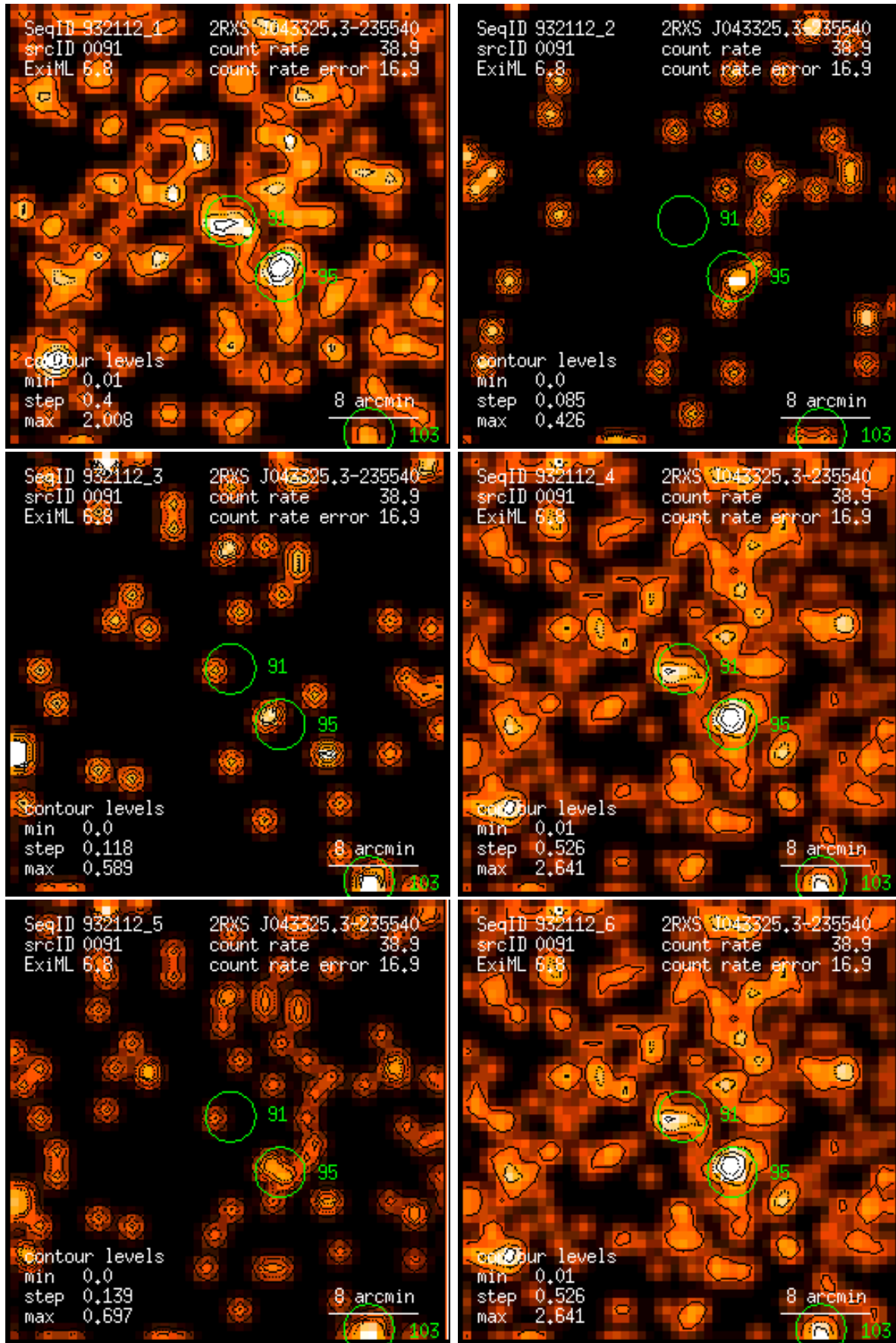
Figure 91: RASS 932112: detection 0091: band rate images, Gaussian filter: (1) PSPC channels 11 – 41, (2) 52 – 90, (3) 91 – 201, (4) 11 – 235, (5) 52 – 201, (6) 11 – 201. Broad band rates in counts/ks. Band rate contour levels in counts/ks/arcmin 2 .
