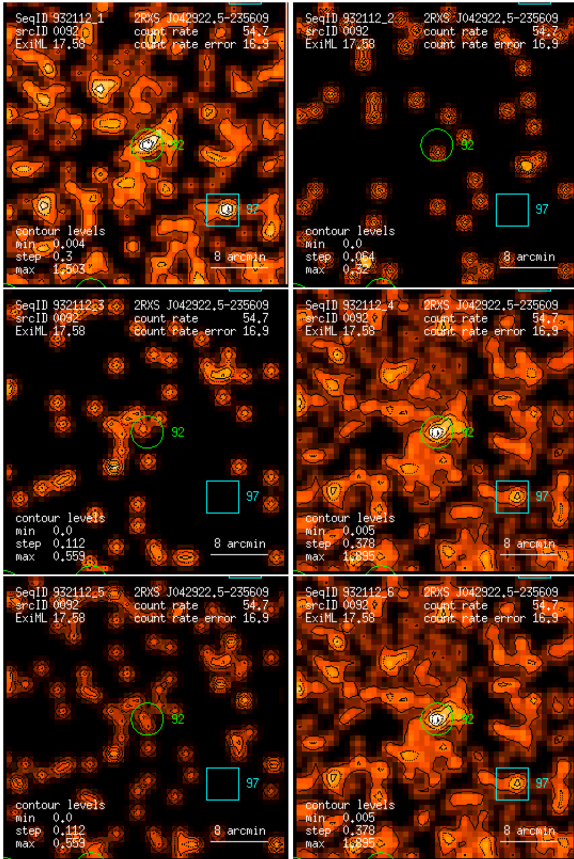
Figure 92: RASS 932112: detection 0092: band rate images, Gaussian filter: (1) PSPC channels 11 – 41, (2) 52 – 90, (3) 91 – 201, (4) 11 – 235, (5) 52 – 201, (6) 11 – 201. Broad band rates in counts/ks. Band rate contour levels in counts/ks/arcmin 2 .
