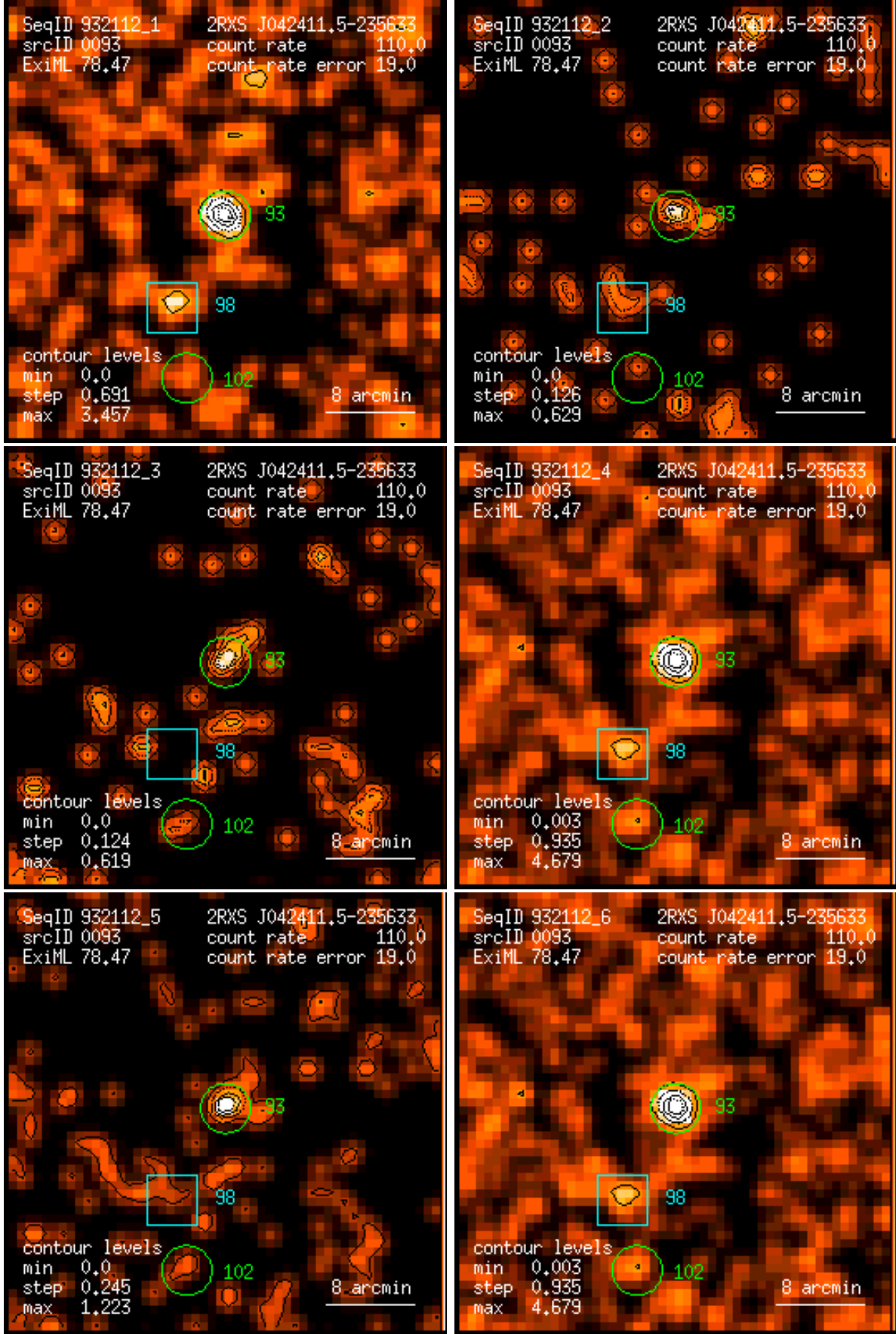
Figure 93: RASS 932112: detection 0093: band rate images, Gaussian filter: (1) PSPC channels 11 – 41, (2) 52 – 90, (3) 91 – 201, (4) 11 – 235, (5) 52 – 201, (6) 11 – 201. Broad band rates in counts/ks. Band rate contour levels in counts/ks/arcmin 2 .
