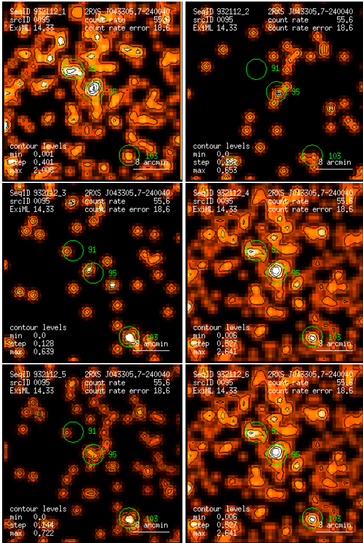
Figure 95: RASS 932112: detection 0095: band rate images, Gaussian filter: (1) PSPC channels 11 – 41, (2) 52 – 90, (3) 91 – 201, (4) 11 – 235, (5) 52 – 201, (6) 11 – 201. Broad band rates in counts/ks. Band rate contour levels in counts/ks/arcmin 2 .
