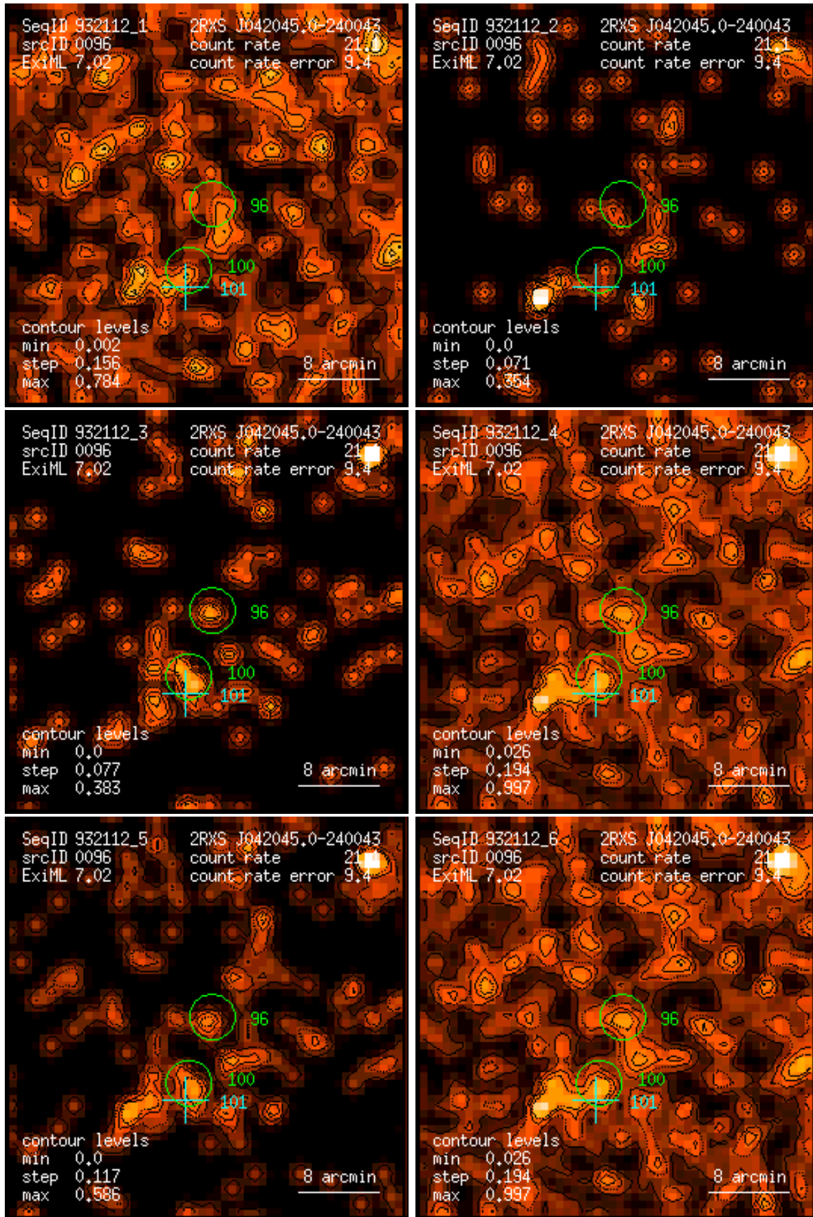
Figure 96: RASS 932112: detection 0096: band rate images, Gaussian filter: (1) PSPC channels 11 – 41, (2) 52 – 90, (3) 91 – 201, (4) 11 – 235, (5) 52 – 201, (6) 11 – 201. Broad band rates in counts/ks. Band rate contour levels in counts/ks/arcmin 2 .
