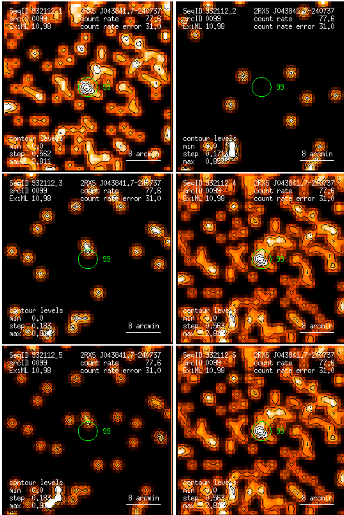
Figure 99: RASS 932112: detection 0099: band rate images, Gaussian filter: (1) PSPC channels 11 – 41, (2) 52 – 90, (3) 91 – 201, (4) 11 – 235, (5) 52 – 201, (6) 11 – 201. Broad band rates in counts/ks. Band rate contour levels in counts/ks/arcmin 2 .
