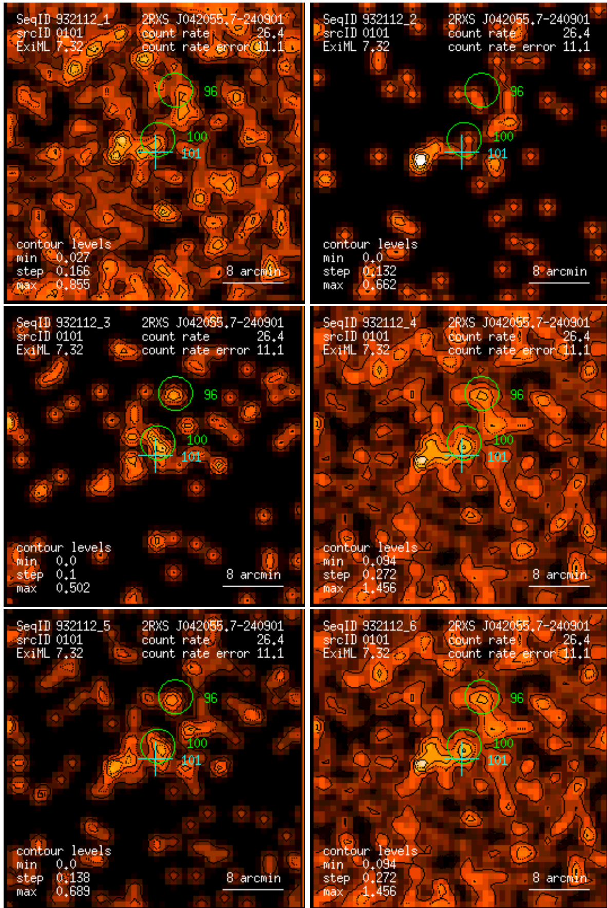
Figure 101: RASS 932112: detection 0101: band rate images, Gaussian filter: (1) PSPC channels 11 – 41, (2) 52 – 90, (3) 91 – 201, (4) 11 – 235, (5) 52 – 201, (6) 11 – 201. Broad band rates in counts/ks. Band rate contour levels in counts/ks/arcmin 2 .
