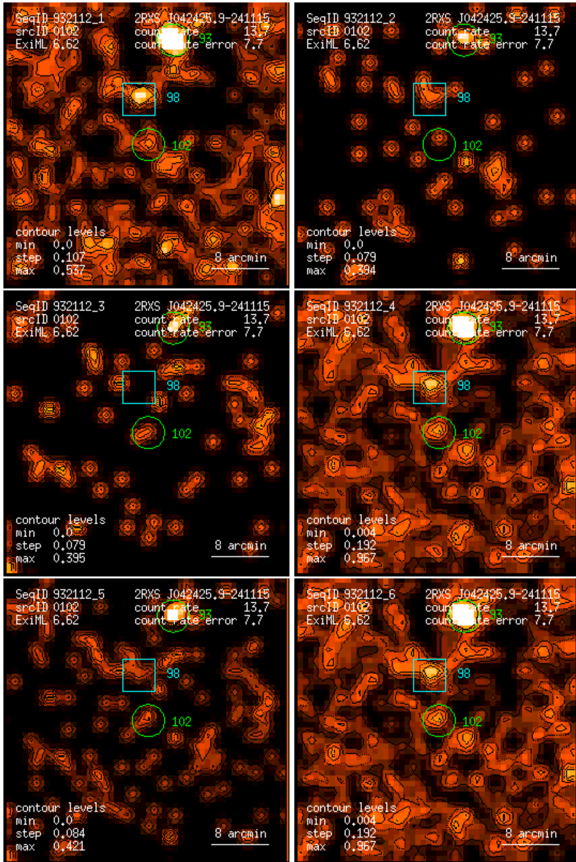
Figure 102: RASS 932112: detection 0102: band rate images, Gaussian filter: (1) PSPC channels 11 – 41, (2) 52 – 90, (3) 91 – 201, (4) 11 – 235, (5) 52 – 201, (6) 11 – 201. Broad band rates in counts/ks. Band rate contour levels in counts/ks/arcmin 2 .
