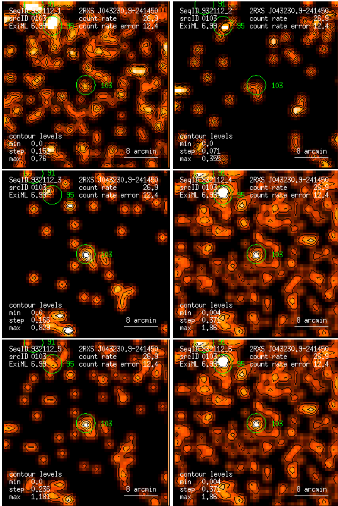
Figure 103: RASS 932112: detection 0103: band rate images, Gaussian filter: (1) PSPC channels 11 – 41, (2) 52 – 90, (3) 91 – 201, (4) 11 – 235, (5) 52 – 201, (6) 11 – 201. Broad band rates in counts/ks. Band rate contour levels in counts/ks/arcmin 2 .
