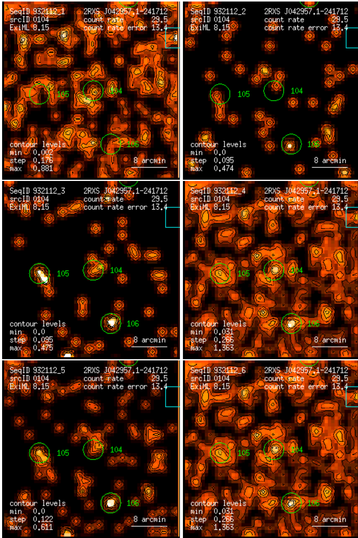
Figure 104: RASS 932112: detection 0104: band rate images, Gaussian filter: (1) PSPC channels 11 – 41, (2) 52 – 90, (3) 91 – 201, (4) 11 – 235, (5) 52 – 201, (6) 11 – 201. Broad band rates in counts/ks. Band rate contour levels in counts/ks/arcmin 2 .
